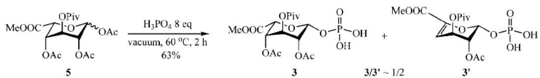
Scheme 3. MacDonal's Phosphorylation of Iduronic Acid Type Donor 5
