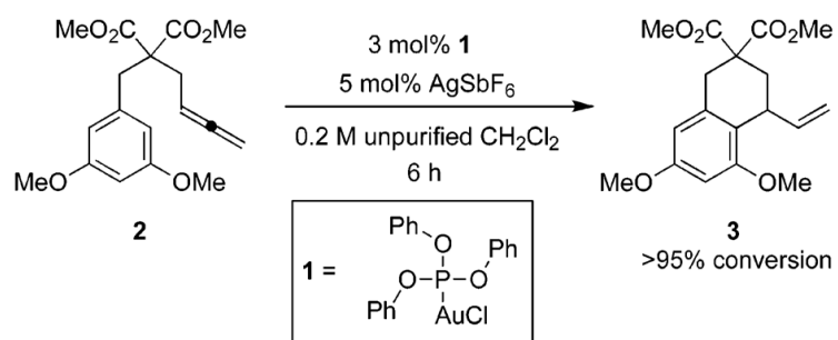
Scheme 3. Optimized Conditions with Activated Substrate 2
