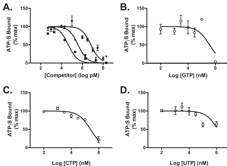
FIGURE 4. NOD2 demonstrates a binding preference for ATP over other nucleotides. A, NOD2 was incubated with 5 nM [^{35}\text{S}]\text{ATP}\gamma\text{S} (17,000 cpm/pmol) and the indicated concentration of unlabeled competitor nucleotides (■, ATP; ▼, dATP; ●, ADP) at 30 °C for 30 min. B–D, NOD2 was incubated with 5 nM [^{35}\text{S}]\text{ATP}\gamma\text{S} (17,000 cpm/pmol) and the indicated concentrations of unlabeled competitor nucleotides: GTP (B), CTP (C), or UTP (D), at 30 °C for 30 min. Bound ATP \gamma S was then assessed as described in Fig. 2. Data points show mean and S.D. (error bars) of triplicate or quadruplicate measurements. Plots are representative of at least three experiments. Curves represent best nonlinear regression fit to a single-site competition model ( y = 100 / (1 + 10^{(x - \log \text{IC}_{50})}) ).
