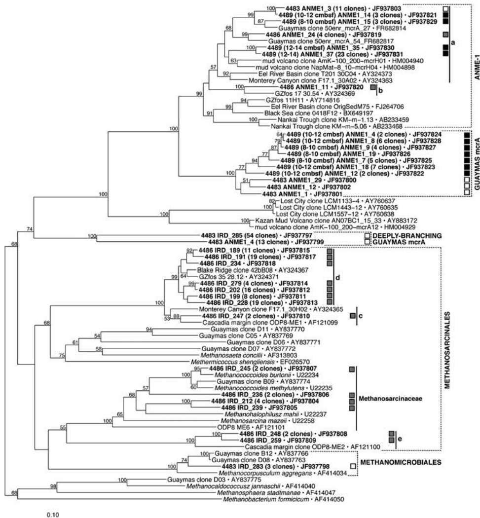
Figure 3 Neighbor-joining distance phylogeny of mcrA genes from Guaymas Basin hydrothermal sediment cores at 15–20°C (open squares), 30–35°C (grey squares) and 60–95°C (black squares). Clones previously found at Guaymas Basin are included for context. Bootstrap values over 50% based on 1000 replicates are shown.
