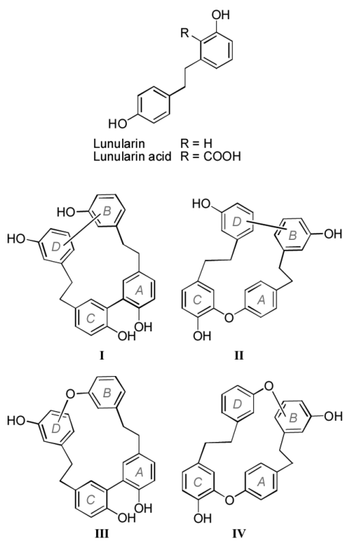
Figure 1. Four distinct structural types of macrocyclic bisbibenzyls.
