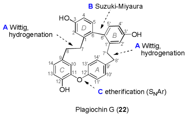
Figure 2. Construction unit system for the synthesis of plagiochin G.
