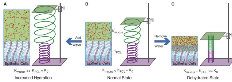
Fig. 5. (A – C) Schematic illustration showing the effects of the relative water-drawing powers of the mucus gel and the PCL
