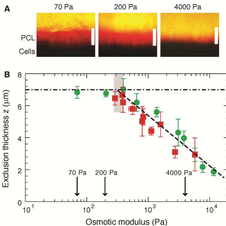
Fig. 4. Osmotic compression of the PCL-brush by mucus and mucus simulants
