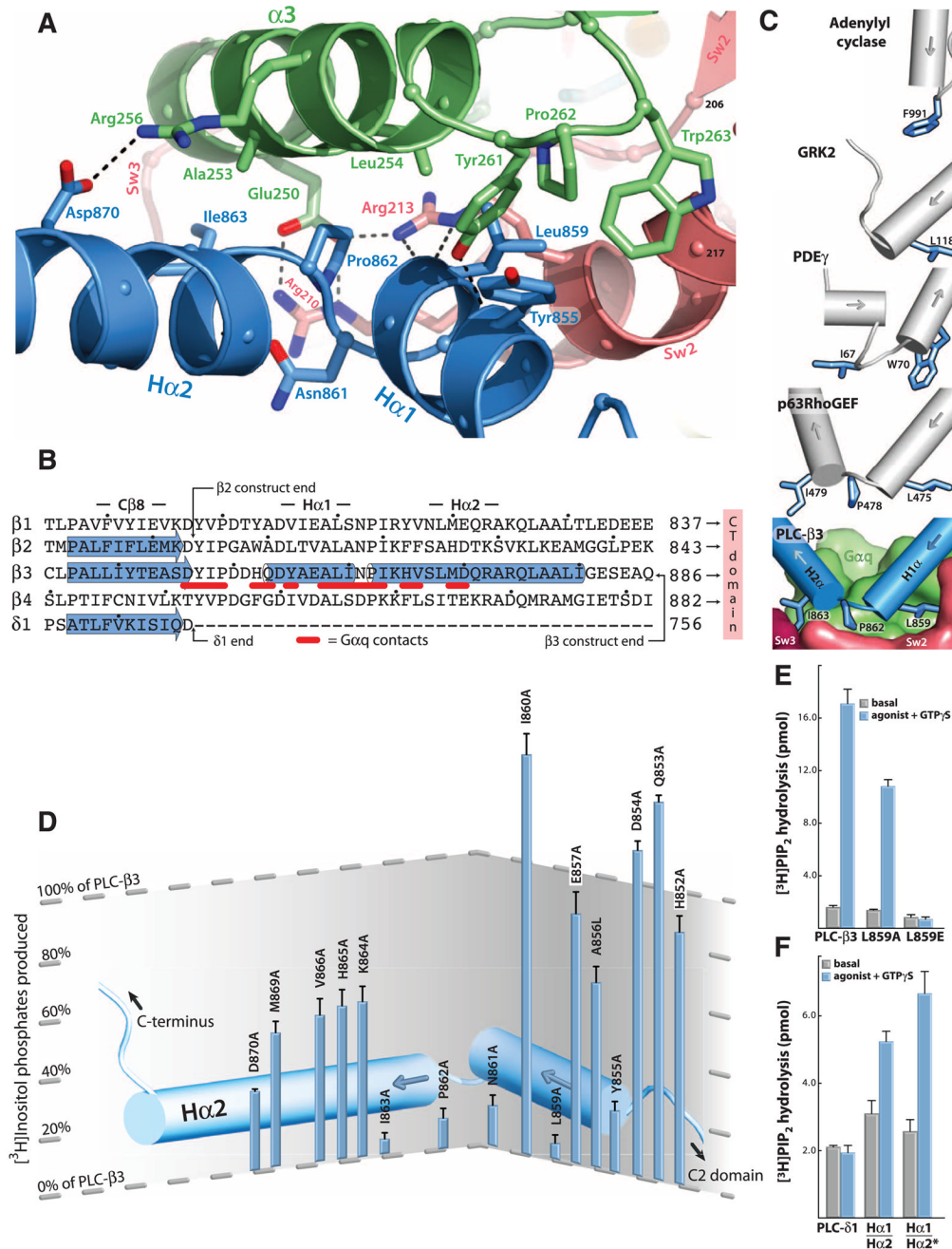
Fig. 2. Structure of the effector binding interface of G\alpha_q •PLC- \beta_3 . (A) Ribbon diagram of the interface between the H\alpha_1/H\alpha_2 region of PLC- \beta_3 (blue) and the effector binding pocket of G\alpha_q located between \alpha_3 (green) and Sw2 (pink). Interfacial residues (sticks) are labeled; hydrogen bonds are indicated by dashed lines. (B) Comparison of PLC sequences (21) at the end of the C2 domain (C \beta 8) encompassing H\alpha_1/H\alpha_2 . \alpha helices (cylinders) and \beta sheets (arrows) were assigned by using crystal structures of PLC- \beta_3 as reported here (PDB 3OHM), PLC- \beta_2 (2ZKM), and PLC- \delta_1 (1DJX). C termini are indicated for full-length PLC- \delta_1 as well as the crystallized fragments of PLC- \beta_2 and - \beta_3 . Residues in PLC- \beta_3 that interact with G\alpha_q are underlined in red. Dots indicate every 10th residue. (C) Comparison of
