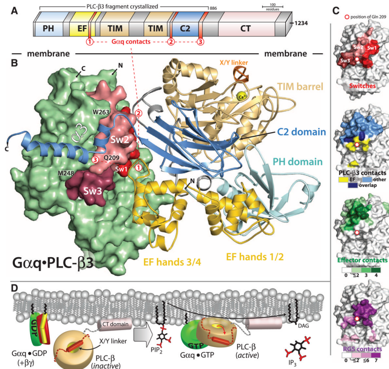
Fig. 1. Structure of G\alpha_q •PLC- \beta_3 . (A) Domain architecture of PLC- \beta_3 drawn to scale and consisting of a N-terminal PH domain, a series of four EF hands, a catalytic TIM barrel, a C2 domain, and a carboxy-terminal (CT) domain. The CT domain is not necessary for G\alpha_q binding (fig. S2), and, therefore, PLC- \beta_3 truncated at residue 886 was used to facilitate crystallization. Three distinct regions of PLC- \beta_3 that interact with G\alpha_q are indicated by red numerals. (B) Overall structure of the AlF_4^- -dependent complex of G\alpha_q •PLC- \beta_3 as viewed from the plane of the membrane. PLC- \beta_3 is depicted as a ribbon cartoon with domains colored as in (A). Activated G\alpha_q is depicted as a green surface with nucleotide-dependent switches (Sw1 to Sw3) in shades of red. Ha1/Ha2 (red 3) at the end of the C2 domain of PLC- \beta_3 lies within the canonical effector-binding region of G\alpha_q formed by \alpha 3 starting at M248 (21), the subsequent loop containing W263, and switch 2 containing Q209. The X/Y linker (orange) connects the two halves of the catalytic TIM barrel, and an ordered portion of the linker occludes the active site of the lipase highlighted by the Ca^{2+} (yellow ball) cofactor. (C) Surfaces of G\alpha_q highlighting switches (top) in comparison to regions (lower images) of G\alpha subunits that interact with PLC- \beta_3 , other effectors, and RGS proteins. Interactions involving the EF3/4 loop are yellow except for overlap (dark blue) involving other regions of PLC- \beta_3 (light blue). G\alpha subunits use a common interface (green) to engage four distinct effectors, and a different interface engages seven distinct RGS proteins (dark purple). Details of the analyses are supplied in (41). (D) Model for activation of PLC- \beta_3 by GTP-activated G\alpha_q . G\alpha_q (green) bound to GDP is sequestered by G\beta\gamma (red and yellow) and does not interact with PLC- \beta_3 , depicted as a gold toroid except for its CT domain (light pink) and X/Y linker (orange cylinder and dotted lines). The CT domain basally associates with membranes, whereas the X/Y linker blocks the lipase active site. Upon activation of heterotrimeric G_q , G\alpha_q -GTP dissociates from G\beta\gamma and interacts with the main portion of PLC- \beta_3 . Complex formation anchors and orients the lipase active site at membranes, leading to repulsion of the X/Y linker and freeing the active site for hydrolysis of PtdIns(4,5) P_2 into diacylglycerol (DAG) and Ins(1,4,5) P_3 (IP _3 ).
