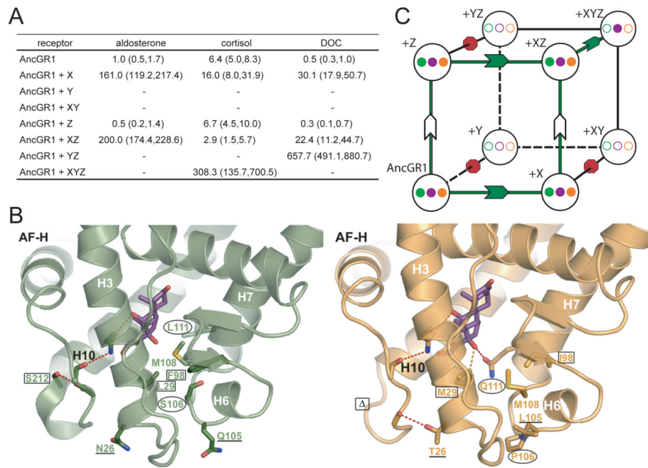
Fig. 3. Permissive substitutions in the evolution of receptor specificity. A ) Effects of various combinations of historical substitutions on AncGR1's transcriptional activity and hormone-response in a reporter gene assay. Group Y (L29M, F98I, and S212 \Delta ) abolishes receptor activity unless groups X (S106P, L111Q) and Z (N26T and Q105L) are present; the XYZ combination yields complete cortisol-specificity. Table shows hormone sensitivity as the EC 50 (in nM). Parentheses, 95% confidence interval. Dash, no activation. B ) Structural prediction of permissive substitutions. Models of AncGR1 (green) and AncGR2 (yellow) are shown with cortisol. Group X and Y substitutions (circles and rectangles) yield new interactions with the C17-hydroxyl of cortisol (purple) but destabilize receptor regions required for activation. Group Z (underlined) impart additional stability to the destabilized regions. C ) Restricted evolutionary paths through sequence space. Nodes of the cube represent states for residue sets X, Y, and Z. Edges represent pathways from the ancestral sequence (AncGR1) to the cortisol-specific combination (+XYZ). Filled circles at vertices show sensitivity to aldosterone (green), DOC (orange), and cortisol (purple); empty circles, no activation. Red octagons, paths through non-functional intermediates; arrows, paths through functional intermediates with no change (white) or switched ligand preference (green).
