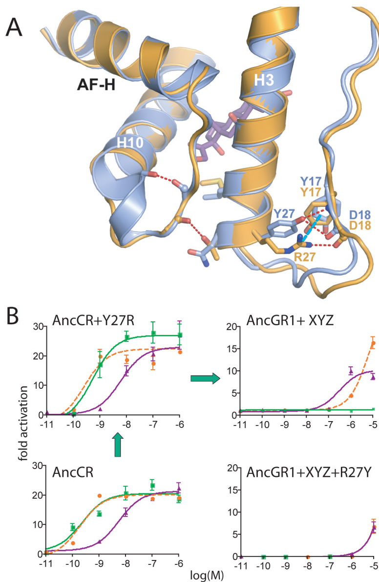
Fig. 4. Structural identification of an ancient permissive substitution. A ) Comparison of the structures of AncCR (blue) and AncGR2 (yellow). Y27R generates a novel cation- \pi interaction in AncGR2 (dotted cyan line), replacing the weaker ancestral hydrogen bond (dotted red) and imparting additional stability to helix 3. B ) Y27R is permissive for the substitutions that confer GR function. Reporter gene activation by AncGR1+XYZ (upper right) is abolished when Y27R is reversed (lower right). Left, Y27R has negligible effect in the AncCR background (or in AncGR1, Fig. S9). Green, orange, and purple lines show aldosterone, DOC, and cortisol response. Green arrows, likely pathway through functional intermediates.
