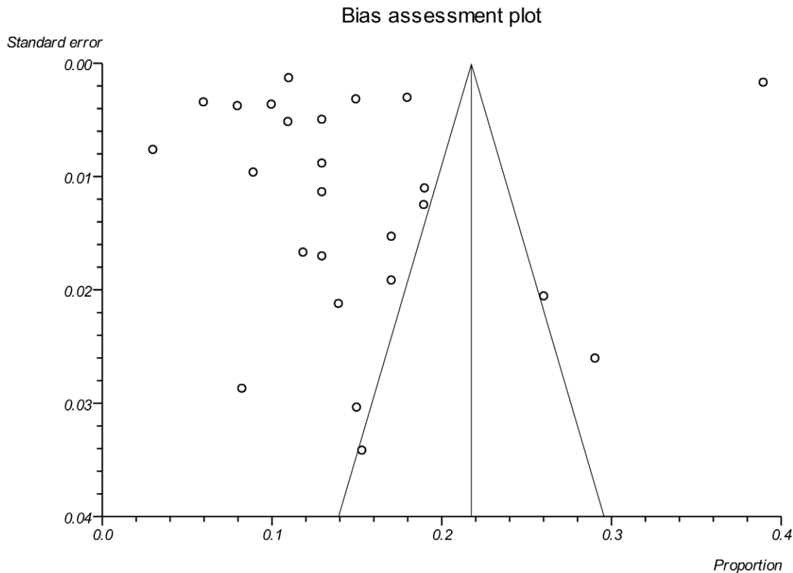
Figure 4. Funnel plot. The funnel plot assesses the hypothesis that the relationship between probability of death and study size, measured by standard error, is independent. This was tested using a Kendall's tau, which was estimated to be 0.4 with p-value = 0.0046, suggesting there is evidence of asymmetry. Although the presence of publication bias is a common explanation to an asymmetric funnel plot, data presented here are observational data without any intervention so the funnel plot asymmetry could also be due to heterogeneity in the data [25]. doi:10.1371/journal.pone.0028691.g004
