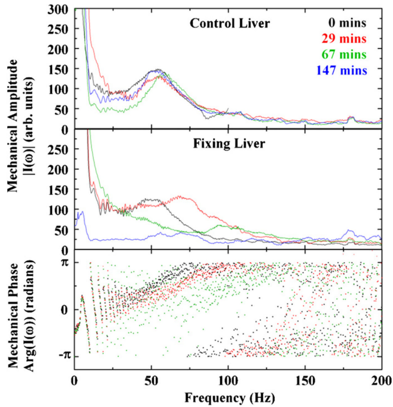
Figure 7. Mechanical resonances with Q \approx 3 are observed in a rat liver, and are used to measure its relative stiffening during formaldehyde fixation. The mechanical spectra of control liver (top panel) and fixing liver (middle and bottom panels) are plotted from 0 to 147 min after exposure to formaldehyde. Results indicate increasing resonant frequency in the fixing liver only, consistent with an increasing Young's modulus.
