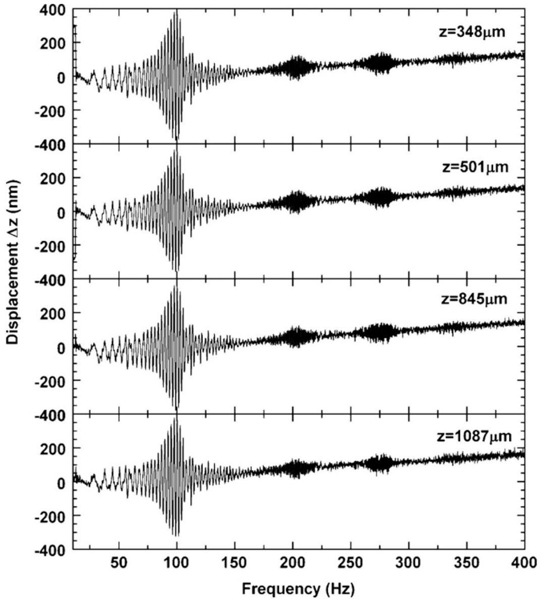
Figure 2. Displacement waveform for an agarose cylinder at varying depths z inside the cylinder demonstrating global vibrations in response to a swept driving frequency. z positions were chosen within equally spaced intervals by selecting the position with the highest OCT signal amplitude, in order to minimize noise.
