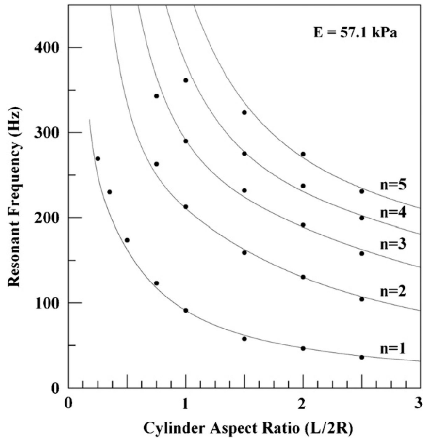
Figure 5. Resonant frequencies in agarose cylinders as a function of their aspect ratio are consistent with the solution for longitudinal modes. Resonant frequency data for modes n = 1, \dots, 5 (where detectible) are plotted with theoretical curves by solving equation (2) using the best-fit Young's modulus E = 57.1 kPa.
