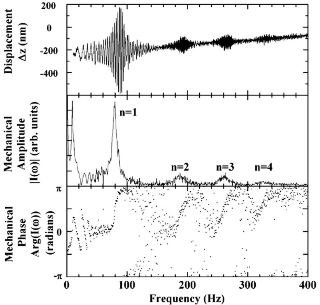
Figure 3. Resonance modes are observed in an agarose cylinder during swept-frequency excitation. Top: raw displacement data versus instantaneous driving frequency. Middle and bottom: computed amplitude and phase, respectively, of the mechanical spectral response \tilde{I}(\omega) . Four longitudinal resonance modes are indicated as n = 1, \dots, 4 . As expected, the phase of \tilde{I}(\omega) shifts from 0 (stress and strain in phase) below each resonance to \pi (stress and strain opposed) above each resonance.
