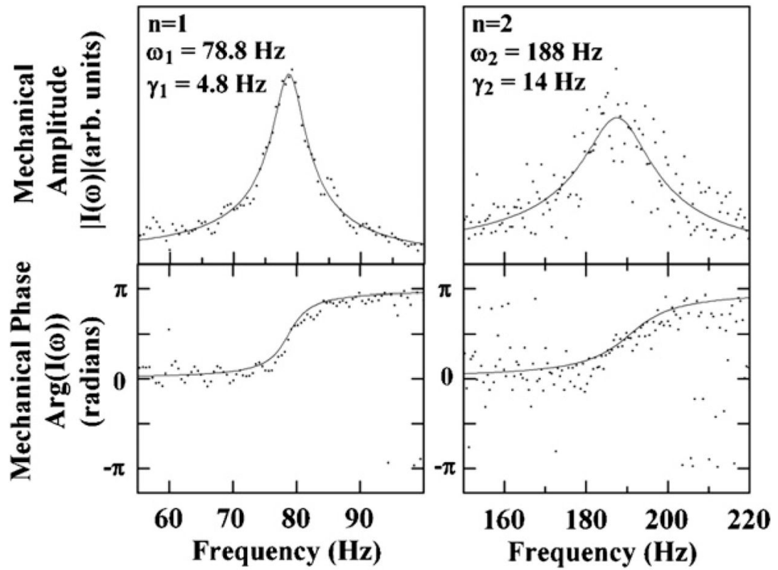
Figure 4. Complex resonance mode data from figure 3 are fit to Lorentzian curves (solid lines) according to equation (3) to determine the resonant frequencies \omega_n and damping factors \gamma_n . Data are shown for n = 1 and 2 (left and right columns, respectively).
