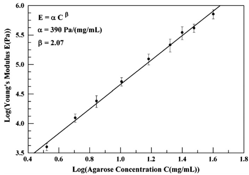
Figure 6. Young's modulus is measured over 2 decades using MRAS in agarose cylinders of varying concentration. Moduli are plotted on a log-log plot and are fit to a phenomenological model (solid line, R^2 = 0.9965 ). Error bars are derived from the half maxima of the resonant frequencies.
