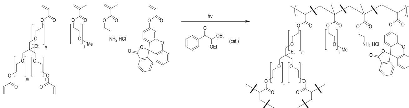
Fig. 1. Chemical structures of monomers and a partial structure of the PRINT particles.
