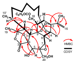
Figure 1. Key HMBC and ^1\text{H} - ^1\text{H} correlations of 6 .
