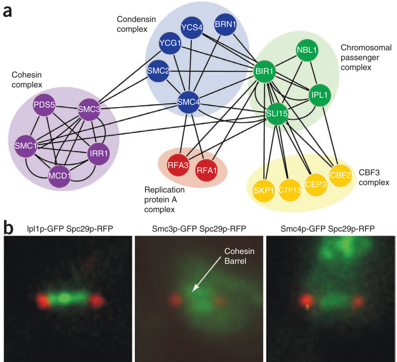
Figure 4. Relationship between cohesin, condensin and chromosomal passenger complexes (CPC). (a) Physical interaction network illustrating protein-protein interactions involving cohesin, condensin and CPC complexes. Nodes represent individual proteins and edges represent physical interactions. (b) Cohesin, condensin and CPC complex localization. Ipl1p-GFP, Smc3p-GFP and Smc4p-GFP localization was assessed with respect to the spindle pole marker, Spc29p-RFP in a wild-type strain. Fluorescent micrograph images illustrate representative single cells.
