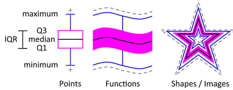
Figure 1. Illustration of boxplots for points, functions, shapes and images. Median (middle black line), confidence region (magenta) and the maximum non-outlying envelope (two outward blue lines). The gray dashed lines are the outliers.
