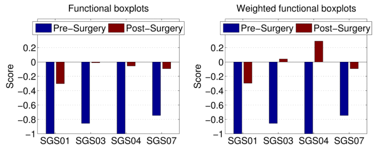
Figure 22. Quantitative comparison of the scores for four SGS subjects before and after surgery using functional boxplots and weighted functional boxplots for atlas-building.
