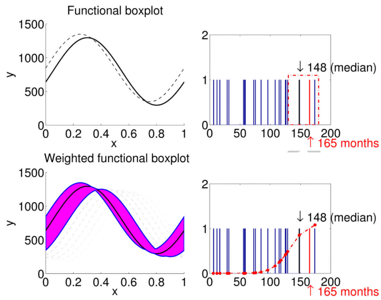
Figure 4. Comparisons of atlases built by the functional boxplot (top) and the weighted functional boxplot (bottom) on the synthetic data. The atlases are built at age 165 months and for both methods the observation at 148 months is selected as the median curve.
