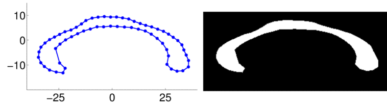
Figure 10. Examples of the corpus callosum shape (left) and the binary image of the corresponding segmentation (right).
