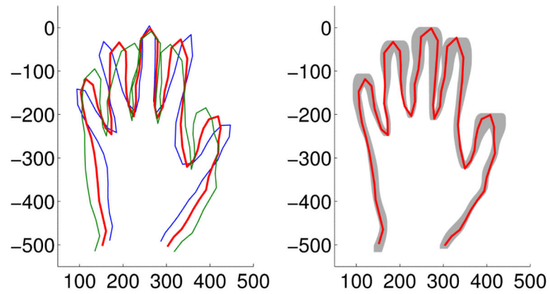
Figure 6. Comparison between the point distribution model (left) and the functional boxplot (right) applied to 18 2D hand contours. Left: mean shape in red and shape variation along the first mode for -3 standard deviations (blue) and for +3 standard deviations (green). Right: median shape in red and 50% confidence region in gray.
