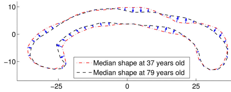
Figure 15. The median shapes of two corpus callosum atlases at different ages and the direction of change of the corresponding points on the boundaries.
