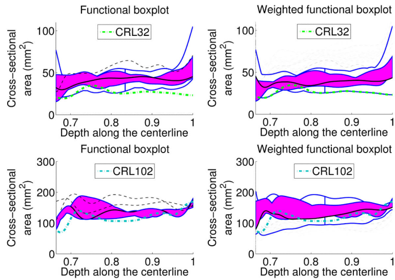
Figure 21. Two control subjects, represented by colored dashed curves and their age-matched atlases. The curves obtain negative scores when using the functional boxplot and non-negative scores when using the weighted functional boxplot.
