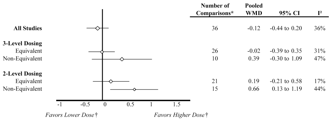
Weighted Mean Difference (WMD) in HAM-D Change from Baseline to Endpoint
