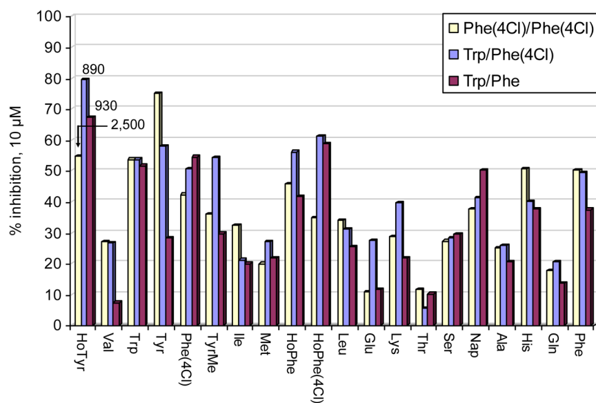
Figure 12. Screening results (% inhibition at 10 \mu M) for the three series of deconvolution compounds against MOR along with measured K_i values (nm) (vs [ 3 H]DAMGO).
