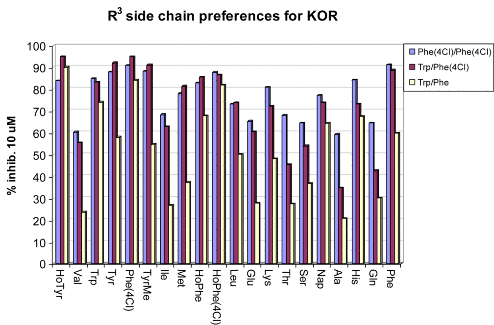
Figure 15. Screening results (% inhibition at 10 \mu M) for the three series of deconvolution compounds against KOR (vs [ 3 H]U69593).
