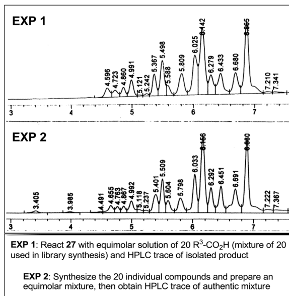
Figure 9. HPLC comparison of library (EXP 1) and authentic (EXP 2) equimolar mixture of final 20 compounds derived from 27. HPLC conditions: linear gradient 0–90% MeCN in H 2 O over 7 min, then 90% MeCN for 10 min at flow rate of 0.75 mL/min.
