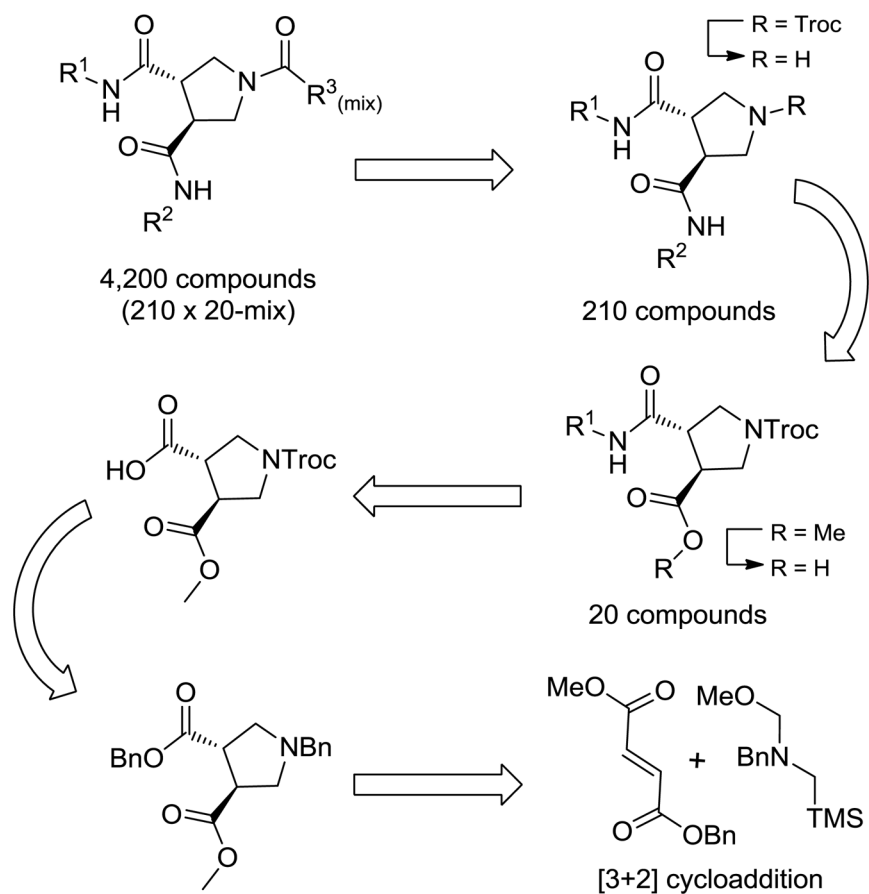
Scheme 1. Retrosynthetic plan for construction of the \beta -turn mimetic library.
