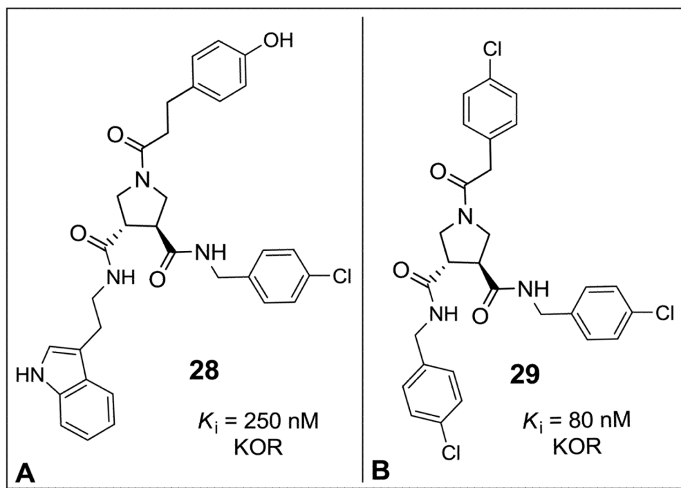
Figure 14. Chemical structures of compounds with highest affinity for KOR from the Trp/Phe(4Cl) series ( 28 ) and the Phe(4Cl)/Phe(4Cl) series ( 29 ).
