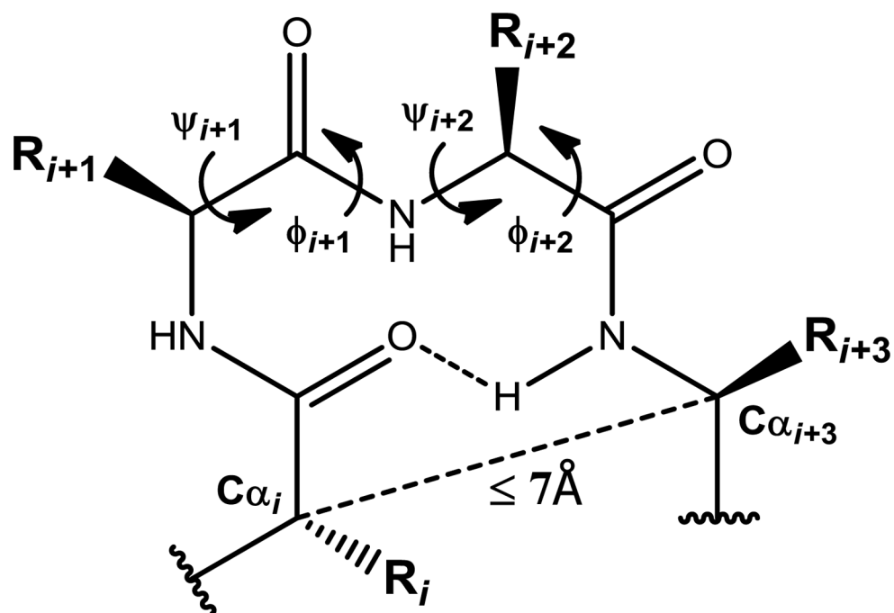
Figure 1. Schematic diagram of a \beta -turn.
