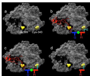
Figure 1. (a) Native C subunit highlighting the active site Cys-199 and its non-active site Cys-343 counterpart. (b) Active site-directed alignment of the maleimide (E) of Caging Agent 1 near Cys-343. (c) Caged C subunit. (d) Photolyzed C subunit. Q = Quencher; F = Fluorophore; ● = PL.
