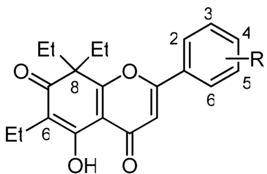
2: 6,8,8-Triethyl-desmodumotin B (TEDB, R = H)
