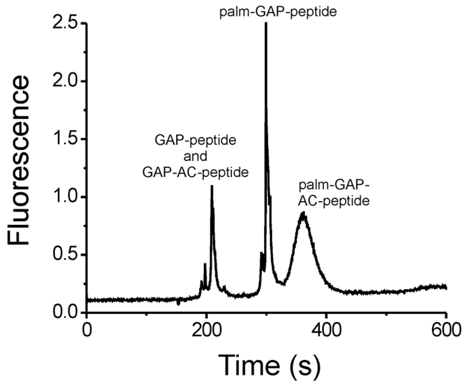
Figure 6. Separation of a mixture of GAP-peptide, GAP-AC-peptide, palm-GAP-peptide, and palm-GAP-AC-peptide in a Tris/CTAB/EtOH electrophoresis buffer.
