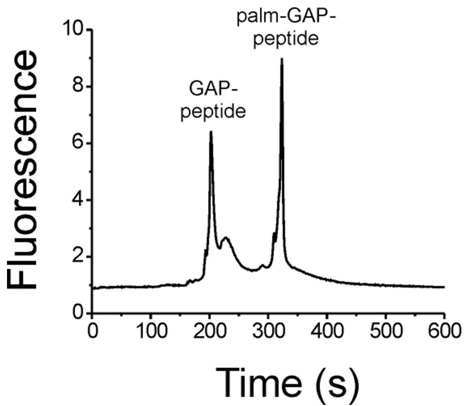
Figure 3. Separation of GAP-peptide and palm-GAP-peptide in tetraborate (25 mM) and CTAB (10 mM). The capillary outlet was held at a positive (+22 kV) potential with the inlet at ground. A bare, 50 \mu\text{m} i.d., fused silica capillary was used.
