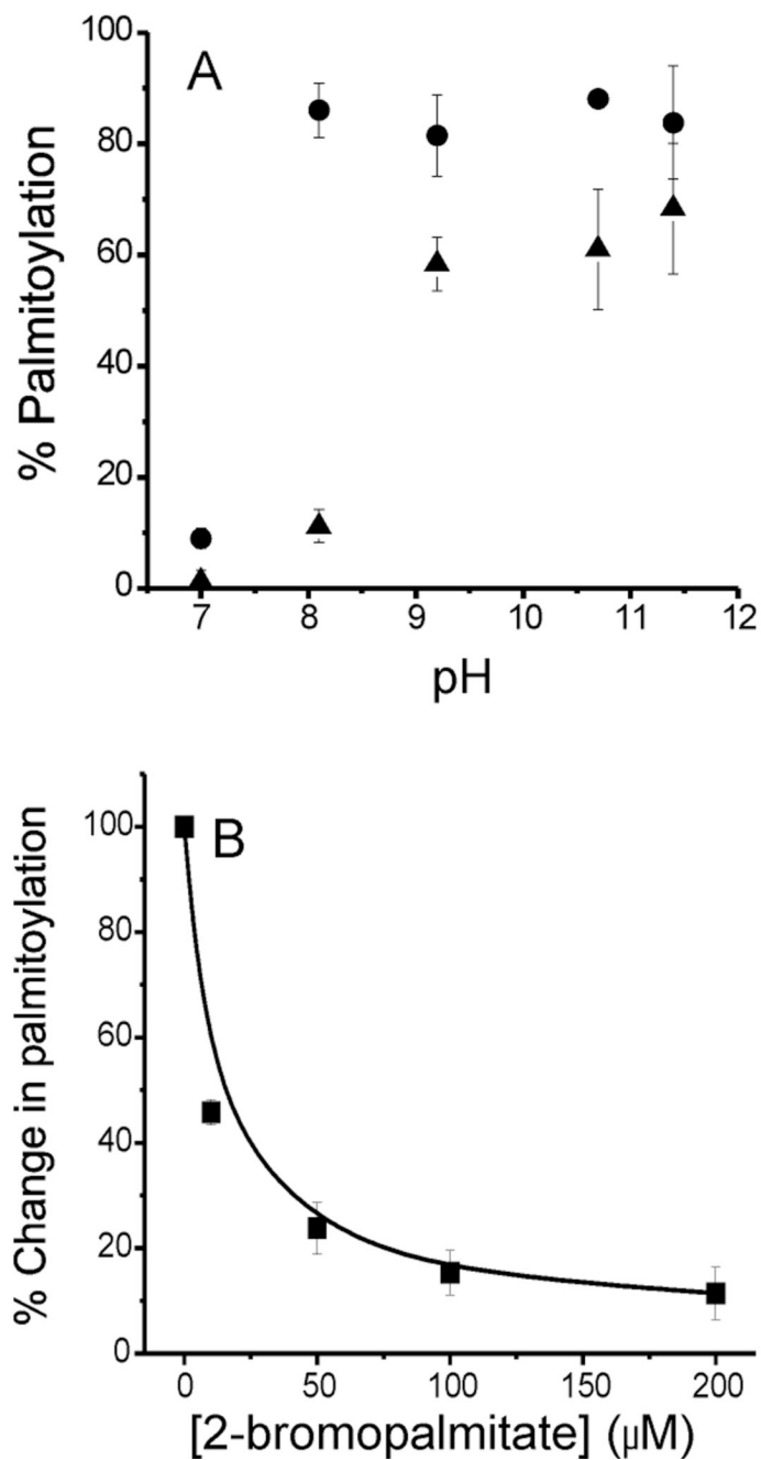
Figure 7. Factors affecting non-enzymatic GAP-peptide palmitoylation. A) Dependence of GAP-peptide palmitoylation on pH (solid circles) and the effect of increasing pH on GAP-peptide palmitoylation in the presence of 200 \mu M 2-BP (solid triangles). B) Inhibition of palmitoylation by 2-bromopalmitate (2-BP). Each point is an average \pm standard deviation of 3 trials.
