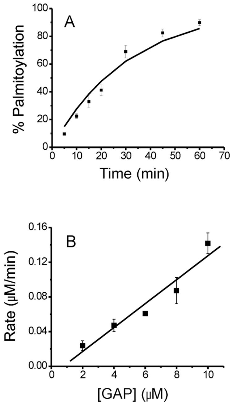
Figure 5. Time dependence and rate of GAP-peptide palmitoylation. A) Time dependence of GAP-peptide palmitoylation. Each point represents the % palmitoylation \pm standard error ( n = 5 ). B) Dependence of GAP-peptide palmitoylation on the GAP-peptide concentration. Each point is an average \pm s.d. ( n=3 ).
