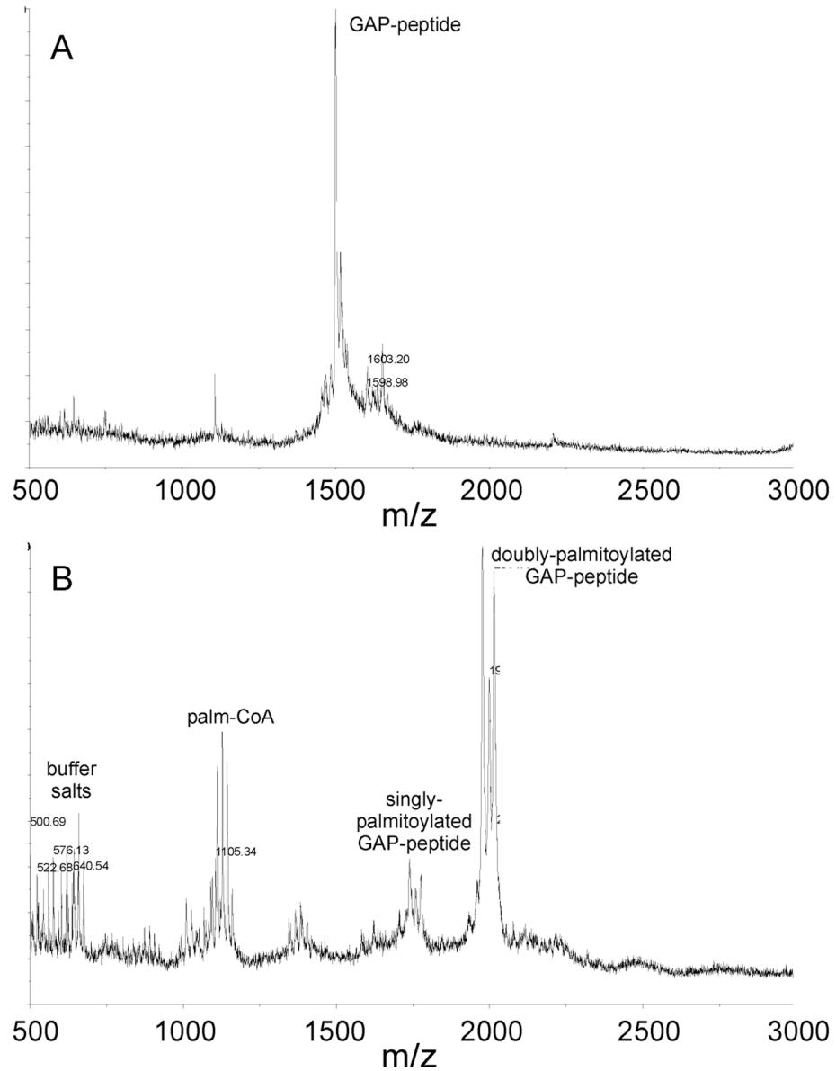
Figure 1. MALDI-MS spectra of A) the GAP-peptide substrate and B) a mixture of GAP-peptide with an excess of palmitoyl coenzyme A after incubation at 37°C for 4 hrs.
