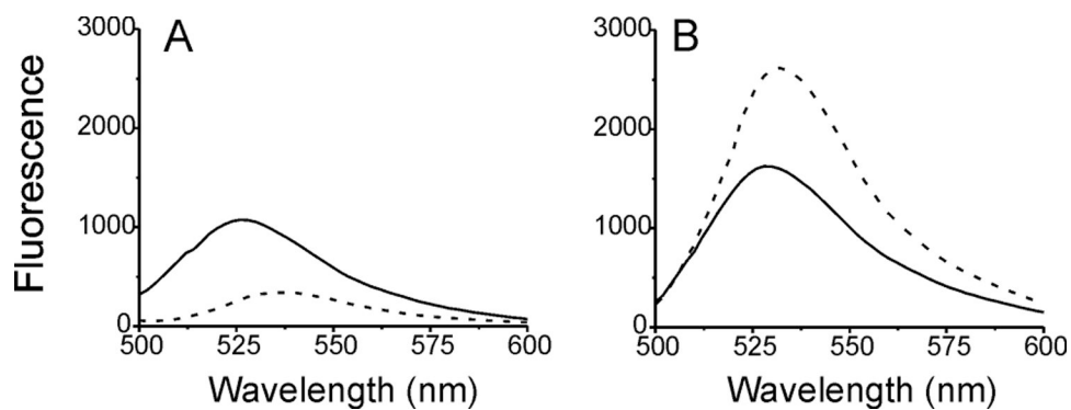
Figure 2. Fluorescence spectra of GAP-peptide substrate and palmitoylated GAP-peptide product. GAP-peptide (solid line) and palm-GAP-peptide (dashed line) ( 1\mu\text{M} each) were dissolved in A) a neutral aqueous buffer and B) an electrophoretic buffer containing CTAB and excited at 473 nm. Peak areas generated from the fluorescence spectra in (B) were used to correct the peak areas of the GAP-peptide and palm-GAP-peptide for their differing fluorescence intensities.
