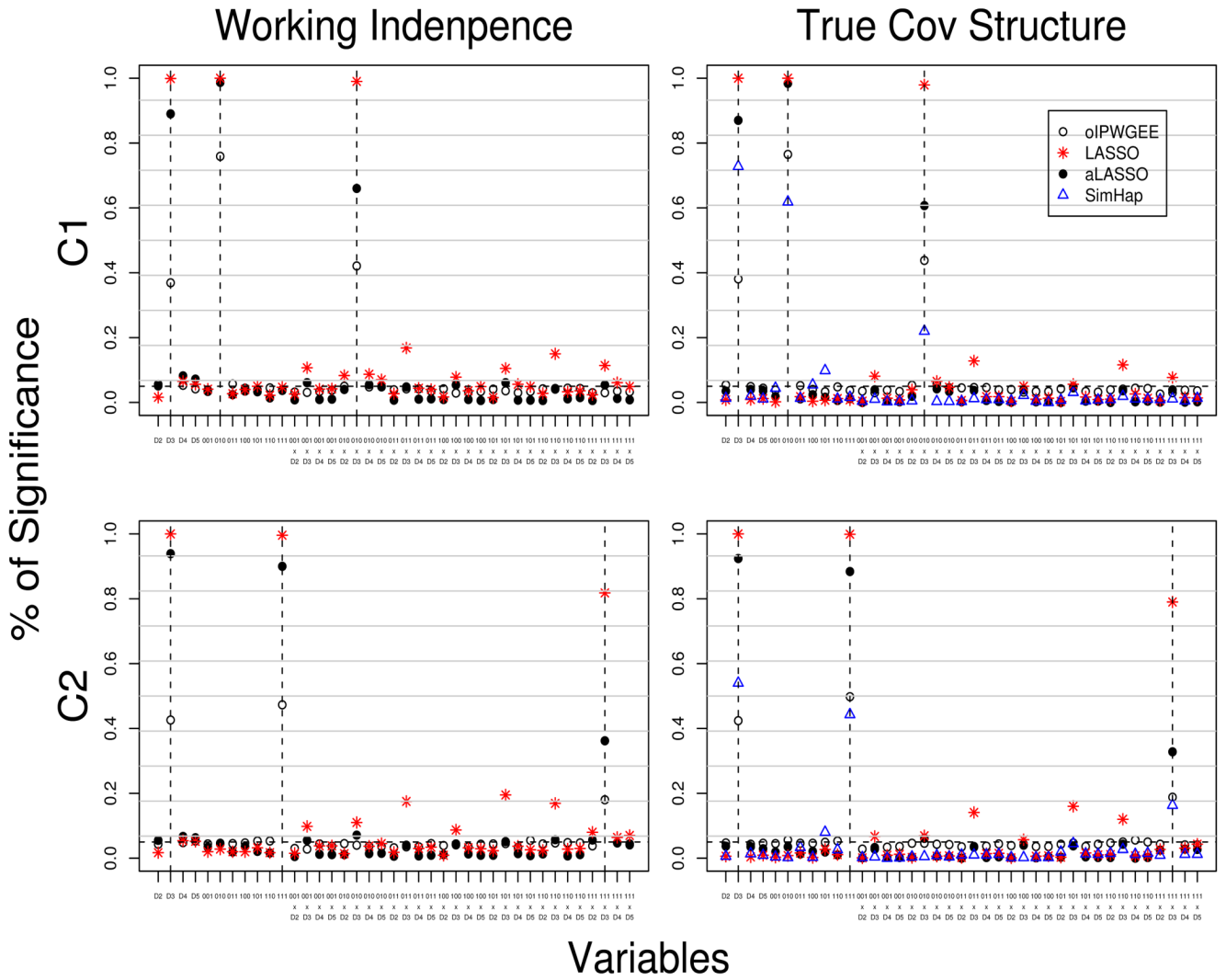
Figure 4. Proportion of significance under Scenario C as defined in Table 1. The left panel shows the results of the proposed IPWGEE methods (i.e., oIPWGEE, LASSO, aLASSO) when a working independence covariance is used, and the right panel shows the results of the IPWGEE and SimHap analysis when the true covariance structure is used. The horizontal dashed line indicates the nominal level of 0.05 used for the Wald test in oIPWGEE and SimHap. The vertical dashed lines indicate the causal effects.
