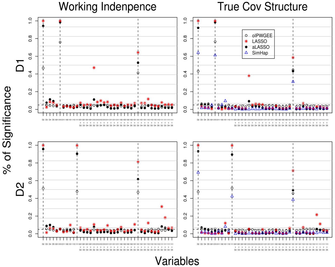
Figure 5. Proportion of significance under Scenario D as defined in Table 1. The left panel shows the results of the proposed IPWGEE methods (i.e., oIPWGEE, LASSO, aLASSO) when a working independence covariance is used, and the right panel shows the results of the IPWGEE and SimHap analysis when the true covariance structure is used. The horizontal dashed line indicates the nominal level of 0.05 used for the Wald test in oIPWGEE and SimHap. The vertical dashed lines indicate the causal effects.
