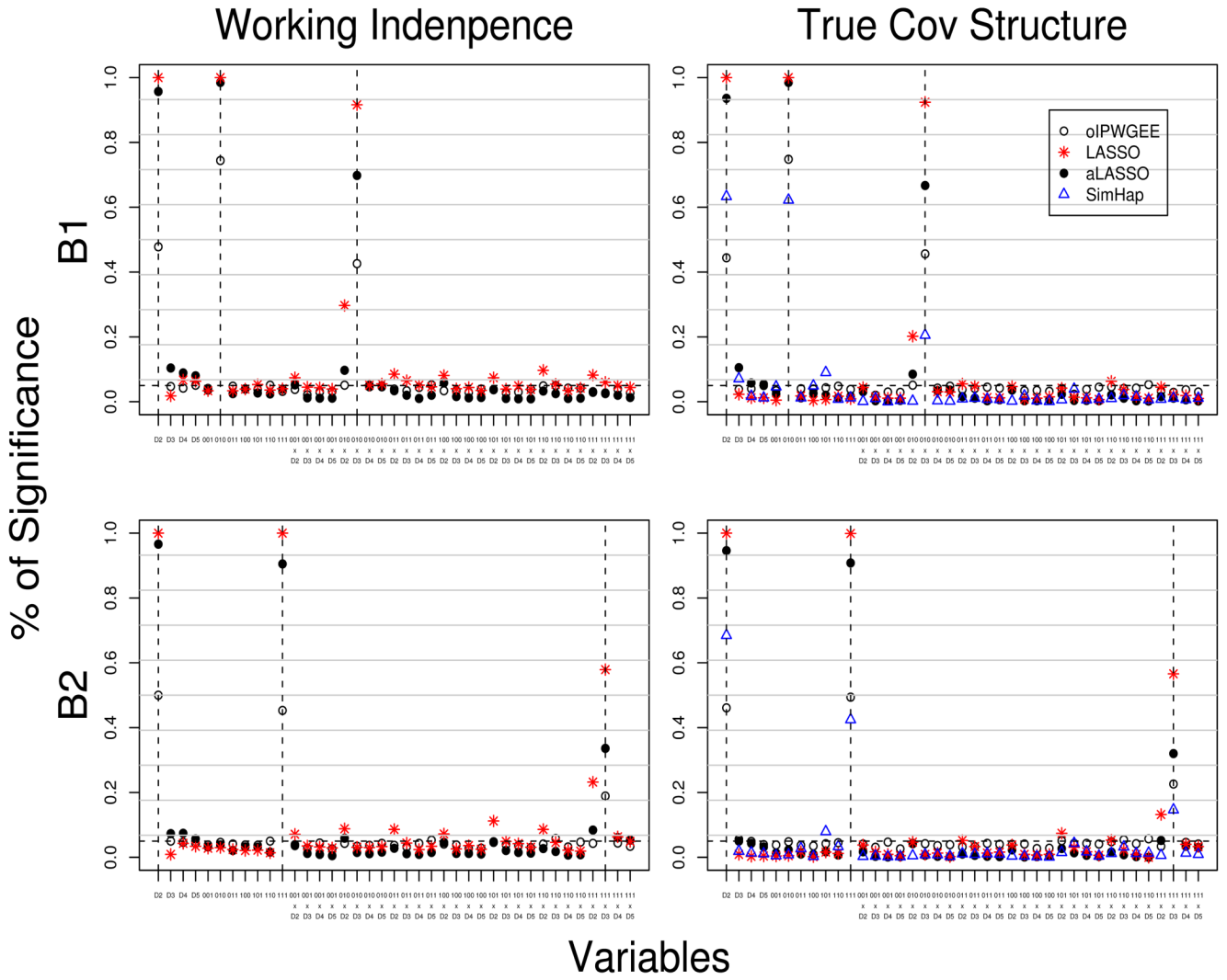
Figure 3. Proportion of significance under Scenario B as defined in Table 1. The left panel shows the results of the proposed IPWGEE methods (i.e., oIPWGEE, LASSO, aLASSO) when a working independence covariance is used, and the right panel shows the results of the IPWGEE and SimHap analysis when the true covariance structure is used. The horizontal dashed line indicates the nominal level of 0.05 used for the Wald test in oIPWGEE and SimHap. The vertical dashed lines indicate the causal effects.
