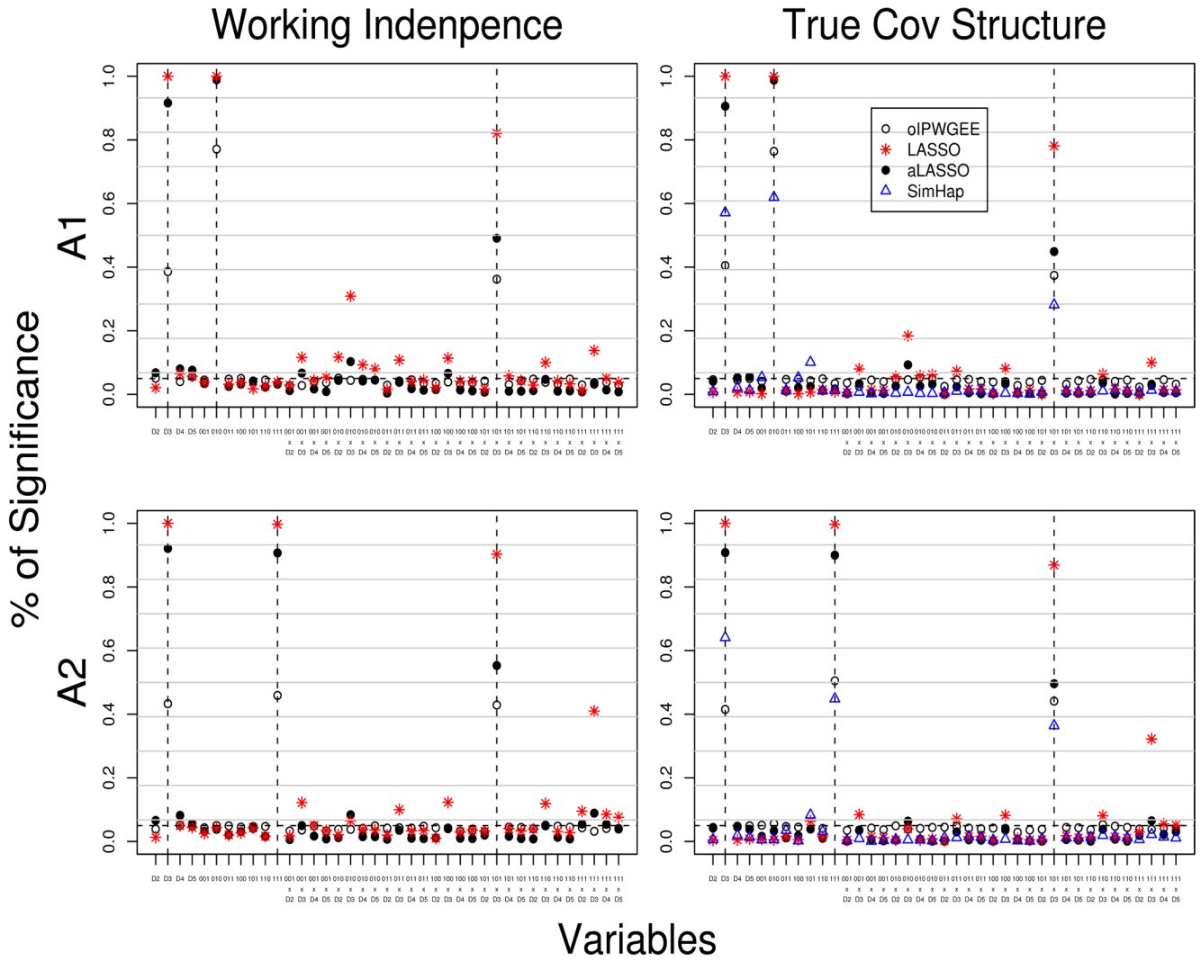
Figure 2. Proportion of significance under Scenario A as defined in Table 1. The left panel shows the results of the proposed IPWGEE methods (i.e., oIPWGEE, LASSO, aLASSO) when a working independence covariance is used, and the right panel shows the results of the IPWGEE and SimHap analysis when the true covariance structure is used. The horizontal dashed line indicates the nominal level of 0.05 used for the Wald test in oIPWGEE and SimHap. The vertical dashed lines indicate the causal effects.
