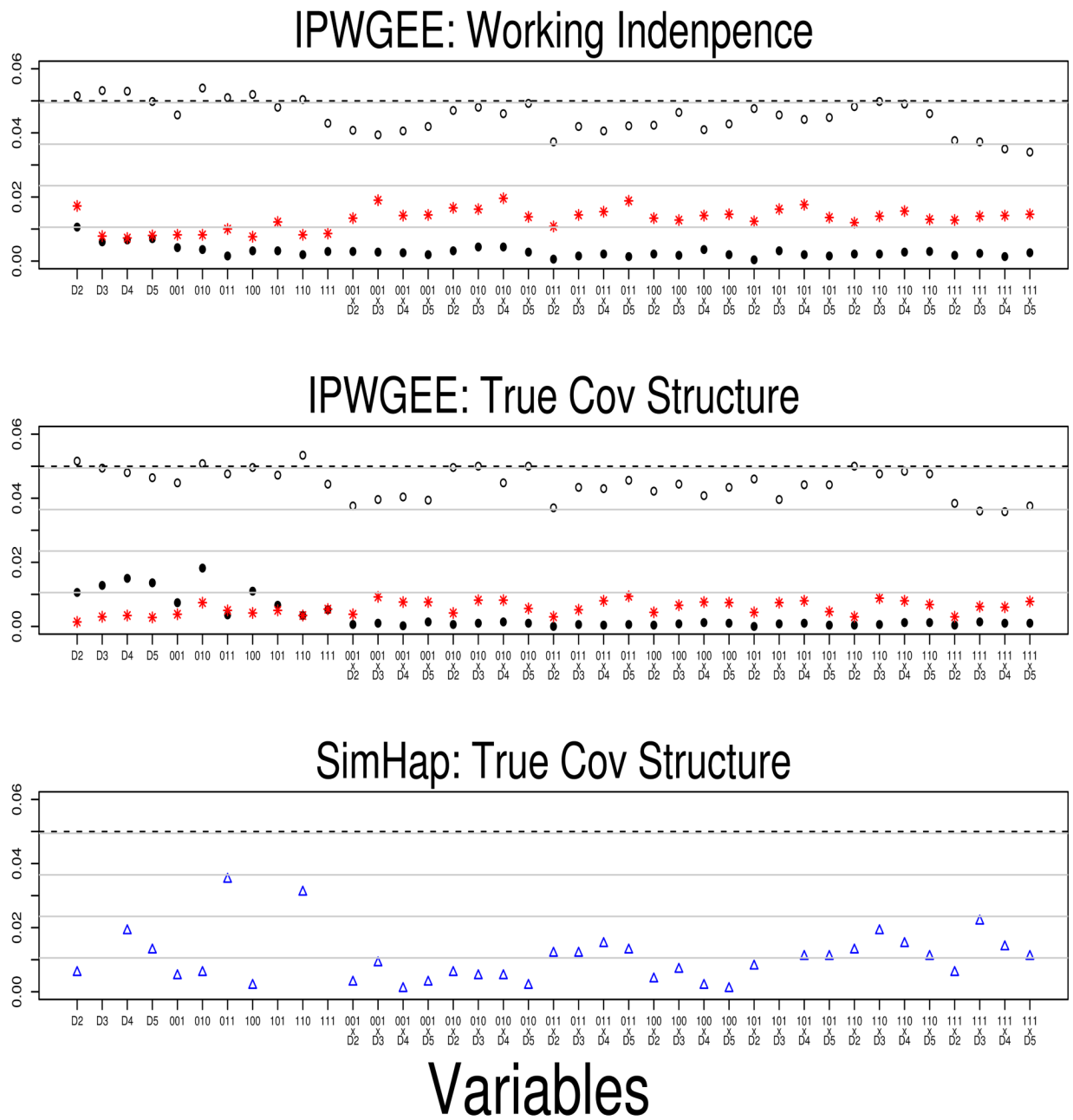
Figure 1. Proportion of significance under the Scenario of ALL NULL (i.e., type I error rates). The top two panels are the results of the proposed IPWGEE methods (i.e., oIPWGEE, LASSO, and aLASSO) with different covariance structures. The open circles, filled circles and the star signs indicate the results for the oIPWGEE, aLASSO and LASSO respectively. The bottom panel is the results of the SimHap, where the type I error rates are indicated by triangles. In all panels, the horizontal dashed line indicates the nominal level of 0.05 used in the oIPWGEE and SimHap methods.
