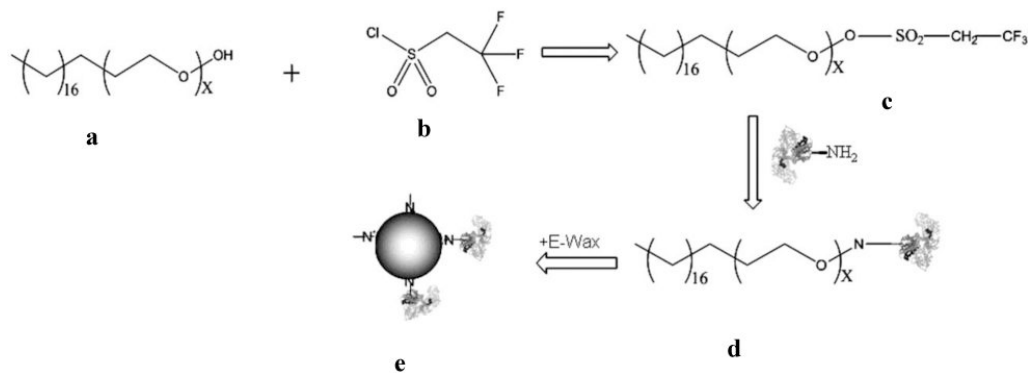
Fig 1. Synthesis and Engineering Scheme for NP-protein formulation. Functionalization of Brij 78 (X=20) & Brij 700 (X=100) (a) by tresyl chloride (b). The resulting T-Brij conjugate (c) was reacted with protein to form Brij 78-protein or Brij 700-protein conjugate (d). The NP-protein (e) was engineered via warm oil-in-water microemulsion precursors using E-wax as oil phase and the synthesized protein conjugate (d) as the surfactant.
