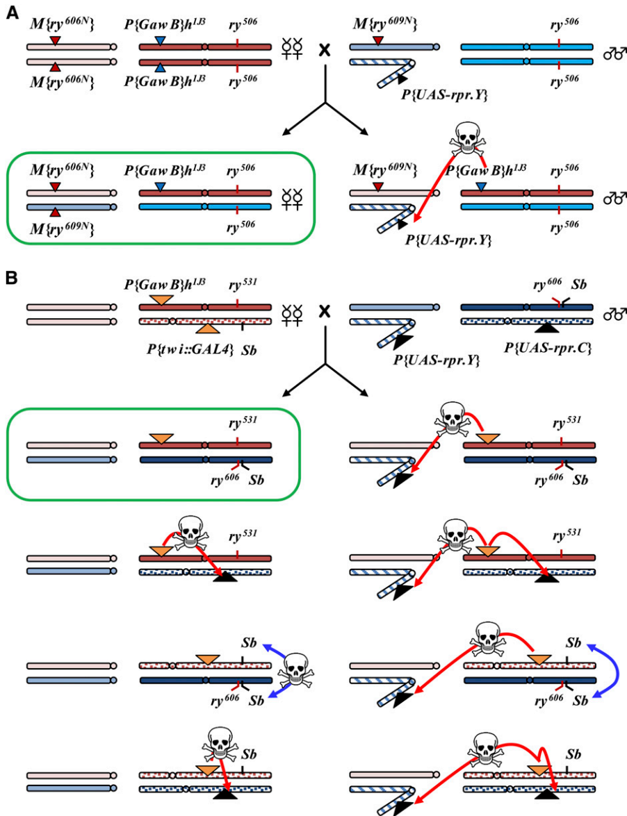
Figure 2 Self-irgining cross schemes. (A) Scheme to generate M\{ry^{606N}\} / M\{ry^{609N}\} virgins. Female chromosomes are red; male chromosomes are blue. Circles indicate centromeres. The Y chromosome is hatched, the telocentric chromosome is the X, and the metacentric chromosome is 3. Triangles denote transgene insertions (the position along the chromosome is not meant to indicate the actual insertion location, which is unknown for some insertions). Genotypes of the parents are represented above, and genotypes of the progeny are shown below. The red arrowhead indicates that Gal4 activates expression of rpr , resulting in death of all sons; only virgin daughters (circled in green) survive. (B) A more complex scheme to generate virgins with a desired heteroallelic combination of third chromosomes. In this cross, eight classes of progeny are produced, four of each sex. Six of these are killed by Gal4-mediated activation of rpr , and seventh dies because of homozygosity for Sb (double-headed blue arrow), leaving only the desired virgin females (circled in green).
