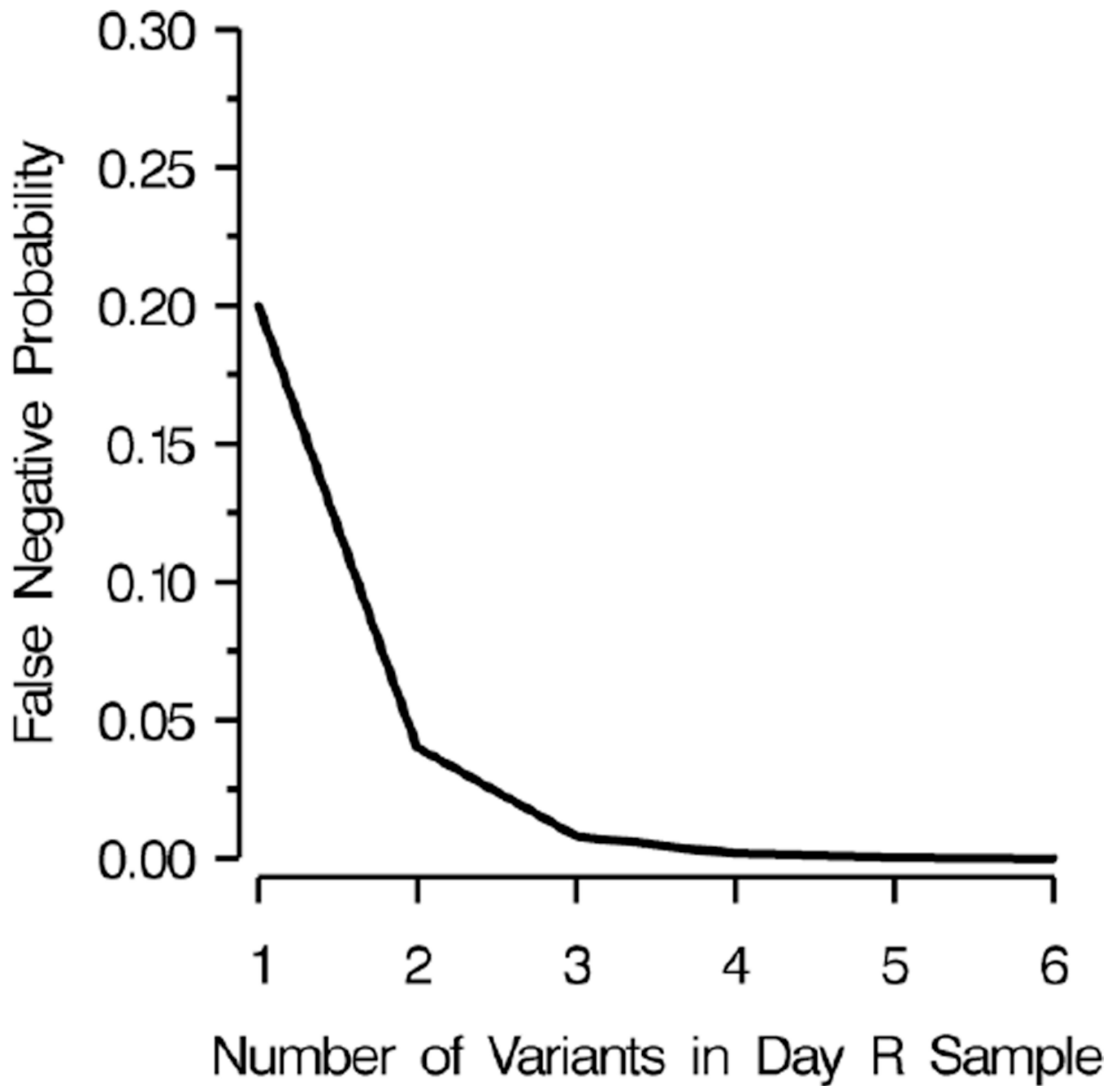
Figure 2. Multiplicity of infection and its effect on the probability of a false negative
