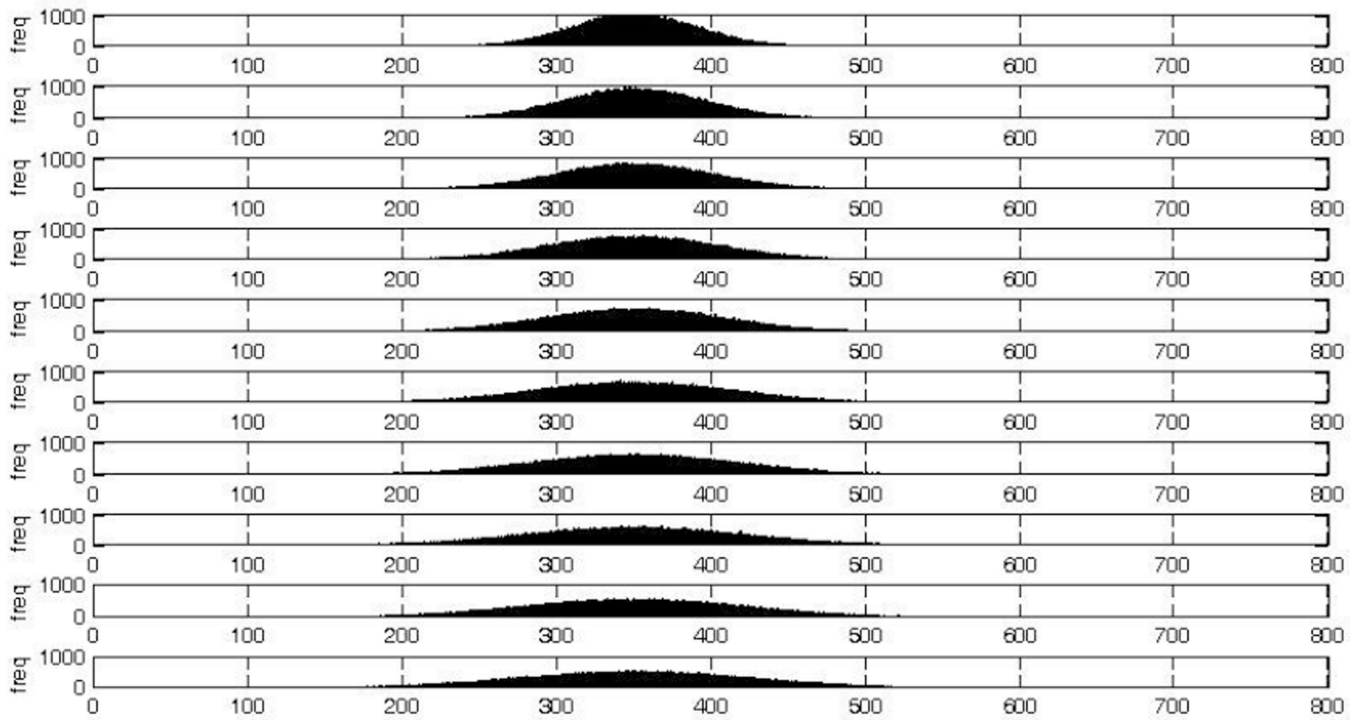
Figure 1. The ten normal distributions of base pairs used for simulations
