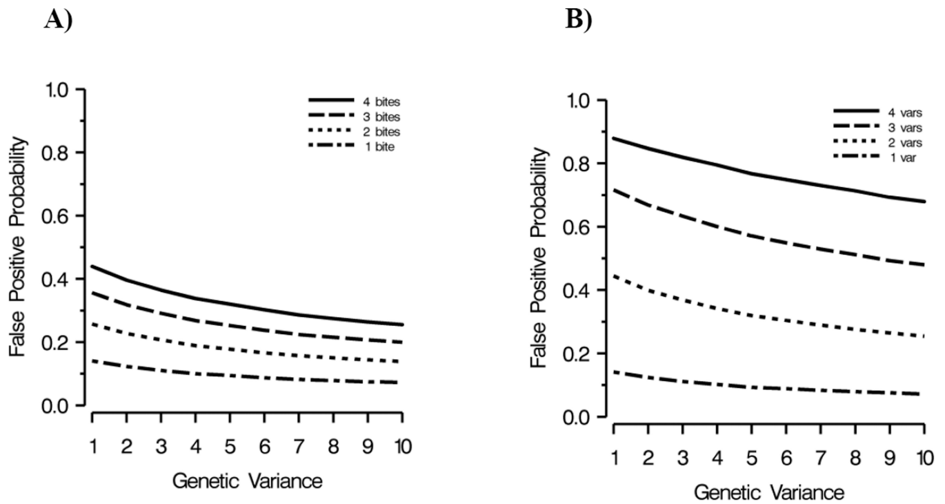
Figure 3. A) The effect of transmission intensity on the probability of a false positive, B) The effect of multiplicity of infection on the probability of a false positive x-axis: measure of allelic variation in parasite population (1 = least variance); y-axis: probability of a false positive (a false positive occurs when a day 0 and day R variant match by chance); var = variant
