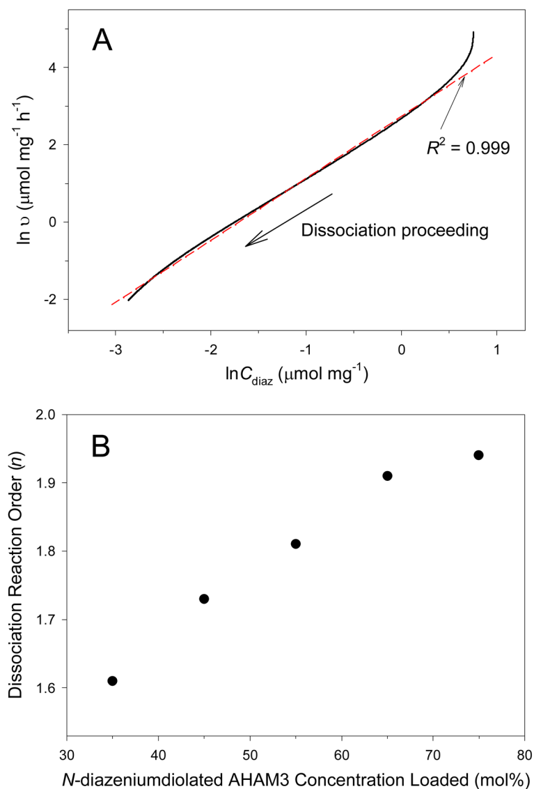
Figure 7. (A) Dissociation kinetic plot of \ln v - \ln C_{\text{diaz}} for 35 mol% N -diazeniumdiolated AHAM3 silica particles (balance TEOS) in deoxygenated PBS (0.01 M, pH 7.4) at 37 °C. The fitting line (dashed red) was determined from a linear regression of the experimental data (solid black). (B) Plot of dissociation reaction order ( n ) versus N -diazeniumdiolated AHAM3 concentration loaded during the silica polymerization.
