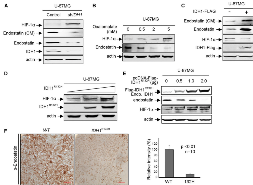
Figure 5. IDH1 Function Supports the Activity of \alpha -KG-Dependent Dioxygenases In Vivo (A–E) The effects of reducing or increasing IDH1 function on two \alpha -KG-dependent dioxygenases, PHDs and C-P4H, were examined in U-87MG cells after knockdown IDH1 (A), treatment of oxalomalate, a competitive inhibitor of IDH1 (B), overexpression of wild-type IDH1 (C), and tumor-derived IDH1 R132H mutant (D and E). The protein levels of HIF-1 \alpha , endostatin, and ectopically and endogenously expressed IDH1 were determined by western blotting. (F) Decreased endostatin in IDH1 R132H gliomas. IDH1 wild-type or heterozygous for R132H glioma samples were subjected to IHC analysis for endostatin. Shown are representative IHC results (left) and mean values of IHC quantification (right). Scale bars represent 50 \mu m. Error bars represent \pm SD for triplicate experiments. Complete results of all 20 samples are presented in Figure S5C. See also Figure S5.
