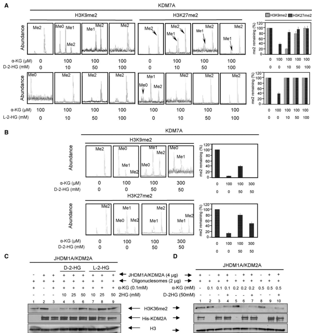
Figure 1. 2-HG Is a Competitive Inhibitor of \alpha -KG for Histone Demethylases (A) 2-HG inhibits Caenorhabditis elegans KDM7A demethylase activity. CeKDM7A activities toward H3K9me2 and H3K27me2 peptides were assayed in the presence of increasing concentrations of either D-2-HG or L-2-HG as indicated. The demethylated products were analyzed by mass spectrometry (left) and mean activity values of duplicated assays, represented by percentage of remaining methylated peptides (right), are shown. Error bars represent \pm standard deviation (SD) for triplicate experiments. (B) \alpha -KG rescues 2-HG inhibition of CeKDM7A demethylase activity. Error bars represent \pm SD for triplicate experiments. (C) 2-HG inhibits human JHDM1A/KDM2A demethylase activity. Purified recombinant JHDM1A demethylase activity was assayed in the presence of various concentrations of D-2-HG and L-2-HG as indicated. (D) \alpha -KG reverses the inhibitory effect of D-2-HG on JHDM1A. JHDM1A activity was assayed in the presence of 50 mM D-2-HG and various concentrations of \alpha -KG. See also Figure S1.
