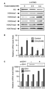
Figure 4. INHIBITION of IDH1 Reduces Histone Demethylase Activities In Vivo (A) Inhibition of IDH1 activity increases histone methylation. Specified histone methylation levels in U-87MG cells treated with increasing concentrations of oxalomalate were analyzed by western blotting. (B and C) Reduction of IDH1 activity activates HOXA genes. HOXA mRNA levels were analyzed by qRT-PCR in U-87MG cells after knocking down IDH1 (C), and treatment of oxalomalate (B). Error bars represent \pm SD for triplicate experiments. See also Figure S4.
