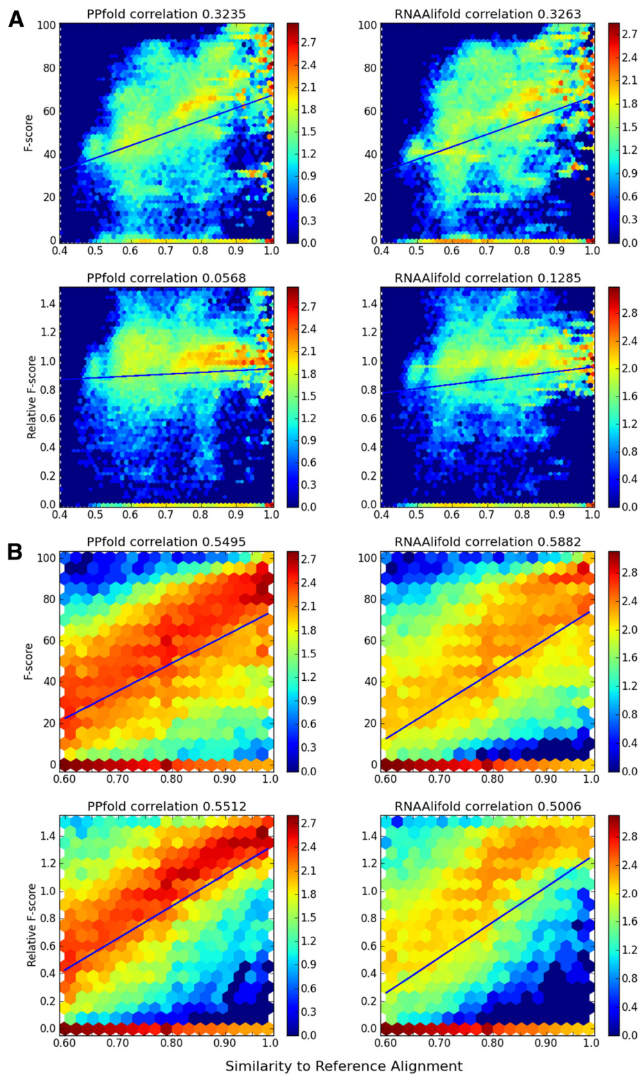
Figure 2 Log-scale heatmaps for mean accuracy, and for percentage of accuracy retained, when alignment quality varies. Performance accuracy on the StatAlign dataset (A) and Random Alignment dataset (B) for PPfold and RNAAlifold when alignment quality is varied. Percentage of accuracy is determined by, for each family, normalising by the average accuracy on the reference alignment. The R^2 correlations given are determined by a linear regression model.
