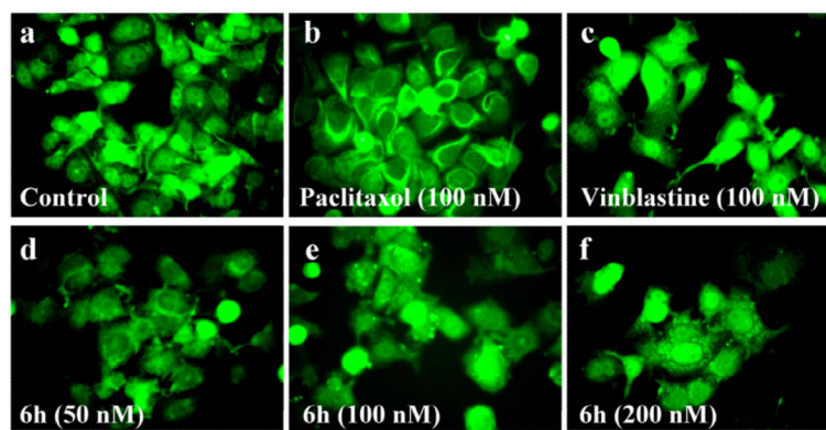
Figure 2. Immunostaining of non-small cell lung cancer NCI-H522 with \alpha -tubulin-FITC. (a) Control; (b) 24 h treatment with paclitaxel at 100 nM; (c) 24 h treatment with vinblastine at 100 nM; (d–f) 24 h treatment with 6h at 50 nM, 100 nM, 200 nM.
