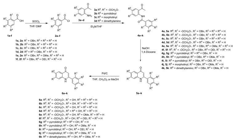
Scheme 1. Synthesis of compounds 6a-k .
