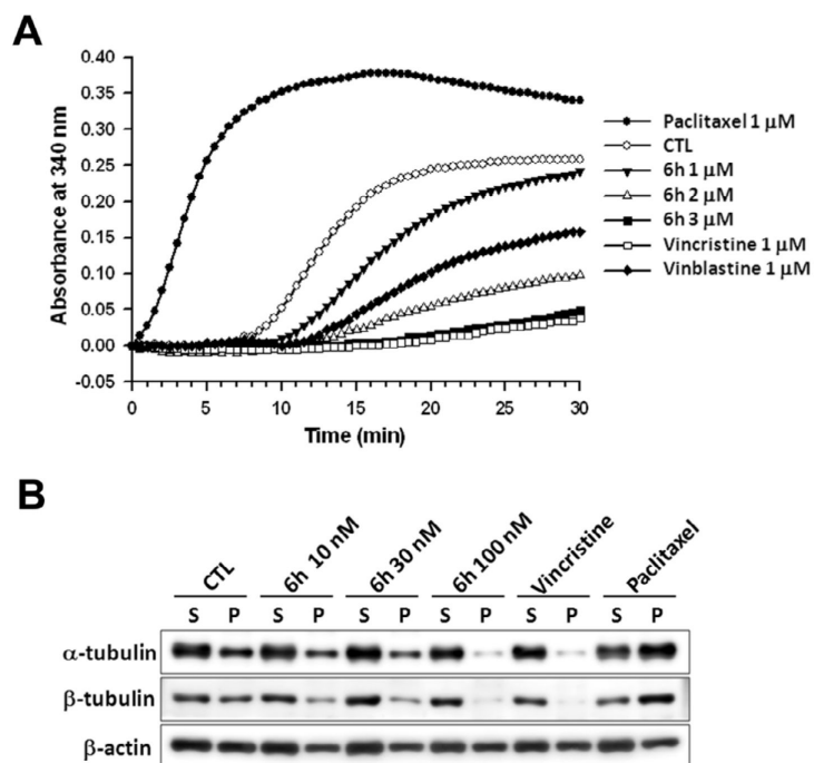
Figure 1. Action mechanism of 6h for anti-proliferation of NCI-H522 non-small cell lung cancer cells. (A) Compound 6h , vincristine, vinblastine, and paclitaxel were incubated with pure tubulin proteins in GPEM buffer. Alteration of tubulin assembly was recorded at absorbance 340 nm. (B) Cells were treated with vehicle (DMSO, as control), 6h (10 nM, 30 nM, and 100 nM), 100 nM vincristine, and 100 nM paclitaxel for 24 h. Cytosolic (S, soluble) and cytoskeletal (P, polymerized tubulin) fractions were separated and followed by Western blot analysis for detection of \alpha -tubulin, \beta -tubulin, and \beta -actin protein expression.
