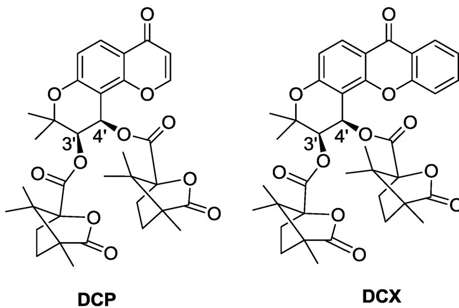
Figure 1. Structures of DCP and DCX.
