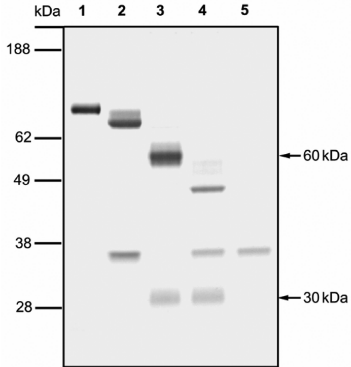
Figure 1. PNGase F treatment of intact and trypsin nicked GGCX
