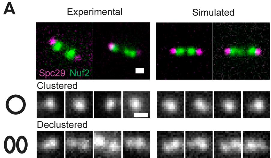
Figure 4. Experimental kinetochore de-clustering is predicted by simulations with a piecewise continuous chromatin spring (CNLS) but not a linear spring (CLS). (A) Experimental and simulated images of WT and mcm21Δ cells with Spc29-RFP (spindle poles) and Nuf2 or Ndc80-GFP (kinetochores) were scored as clustered (kinetochore focus) or declustered in cells having the focus of 16 kinetochores split into multiple foci. Example experimental (left) and simulated (right) images showing a bundle of clustered (middle) and declustered (bottom). (B) Experimental declustering in WT and mcm21Δ cells (WT: 9 \pm 4\% , n = 209 , two experiments; mcm21Δ : 32 \pm 6\% , n = 230 , two experiments). (C and D) Model simulations were used to generate images that match the physical geometry of the mitotic spindle (model convolution; Quammen et al., 2008; Gardner et al., 2010). The position of the spindle poles and plus end of each kMT were convolved with the point-spread function of our microscope objective to produce a simulated image of spindle poles and clusters of kinetochore proteins at the microtubule plus ends. Declustering was scored using the same criteria as in experimental images ( n = 300 , three groups of 100). (C) Decreasing the linear spring constant by an order of magnitude results in an insignificant increase ( 9\text{--}12\% , \chi^2 > 0.30 ) in kinetochore declustering. (D) Decreasing the threshold of a piecewise continuous spring results in a significant increase in declustering ( 10\text{--}22\% , \chi^2 < 1 \times 10^{-4} ) comparable to experimental (B vs. D). Bars, 0.5 \mu\text{m} . Error bars represent standard deviation.
