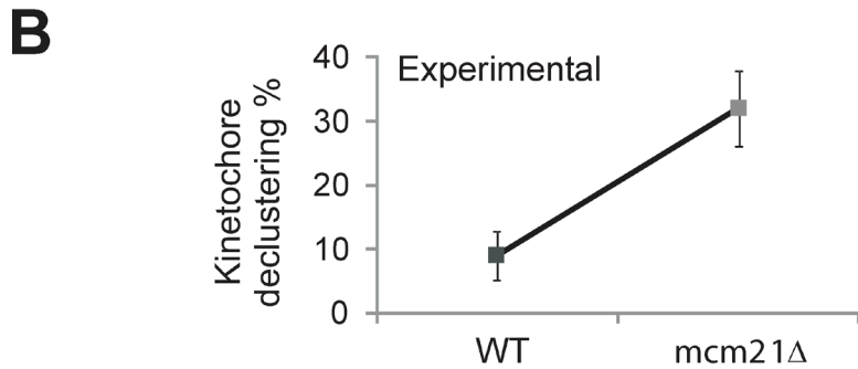
Figure 4. Experimental kinetochore de-clustering is predicted by simulations with a piecewise continuous chromatin spring (CNLS) but not a linear spring (CLS). (A) Experimental and simulated images of WT and mcm21Δ cells with Spc29-RFP (spindle poles) and Nuf2 or Ndc80-GFP (kinetochores) were scored as clustered (kinetochore focus) or declustered in cells having the focus of 16 kinetochores split into multiple foci. Example experimental (left) and simulated (right) images showing a bundle of clustered (middle) and declustered (bottom). (B) Experimental declustering in WT and mcm21Δ cells (WT: 9 \pm 4\% , n = 209 , two experiments; mcm21Δ : 32 \pm 6\% , n = 230 , two experiments). (C and D) Model simulations were used to generate images that match the physical geometry of the mitotic spindle (model convolution; Quammen et al., 2008; Gardner et al., 2010). The position of the spindle poles and plus end of each kMT were convolved with the point-spread function of our microscope objective to produce a simulated image of spindle poles and clusters of kinetochore proteins at the microtubule plus ends. Declustering was scored using the same criteria as in experimental images ( n = 300 , three groups of 100). (C) Decreasing the linear spring constant by an order of magnitude results in an insignificant increase ( 9\text{--}12\% , \chi^2 > 0.30 ) in kinetochore declustering. (D) Decreasing the threshold of a piecewise continuous spring results in a significant increase in declustering ( 10\text{--}22\% , \chi^2 < 1 \times 10^{-4} ) comparable to experimental (B vs. D). Bars, 0.5 \mu\text{m} . Error bars represent standard deviation.
