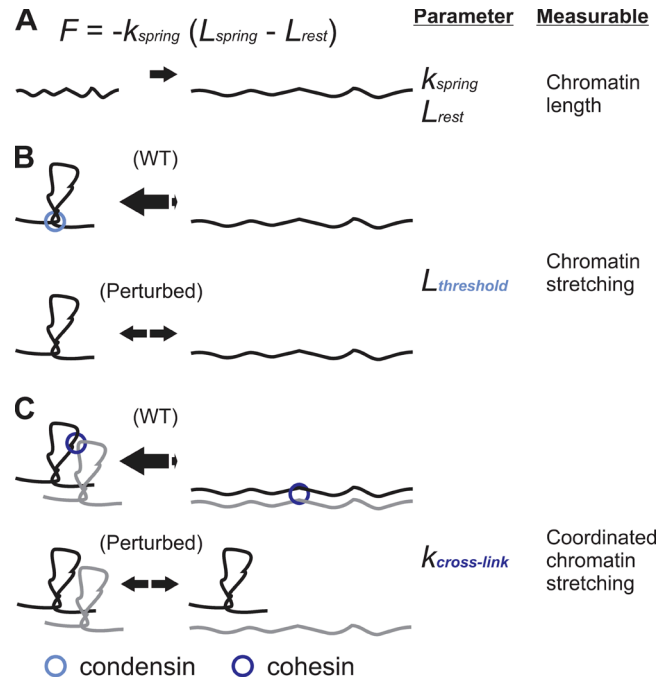
Figure 6. Testable parameters of a piecewise continuous spring. (A) The most common form of a spring is given by a Hookean spring equation F = -k_{spring}(L_{spring} - L_{rest}) , in which k is the spring constant, and L_{rest} is the spring rest length. Simulations of a linear spring fail to account for behavior of the spindle and the pericentric chromatin upon experimental depletion of pericentric cohesin or condensin (see Table 1). (B) A nonlinear spring with a threshold length ( L_{threshold} ) recapitulates increase in spindle length and fluctuations, asymmetric chromatin stretching, and kinetochore declustering. The threshold represents the length/force at which a compact loop transitions to a stretched loop. Cohesin and condensin increase the threshold of the chromatin loops maintaining compaction (equilibrium arrows shifted toward loops). Perturbation of the chromatin spring through depletion of pericentric cohesin or condensin decreases the length/force the loops can resist, causing the loops to stretch freely (equal amounts of compact and stretched loops; Fig. 2, A and C). The L_{threshold} variable is an alternative way to modulate the native linear spring constant ( k ) and rest length ( L_{rest} ). (C) Experimentally observed stretching of two chromosomes could be simulated through the addition of a cross-linking spring between neighboring chromosomes ( k_{cross-link} ; Fig. 5). Cross-linked chromatin springs can distribute tension, thereby increasing the ability of a single chromatin spring to resist reaching L_{threshold} or extreme stretching (equilibrium arrows shifted toward the looped state). Simulation and experimental data suggest condensin and cohesin modulate L_{threshold} and k_{cross-link} , respectively.
