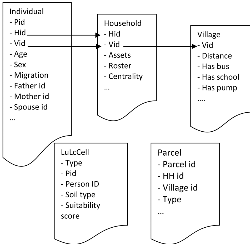
Figure 2. File links between social agents in the ABM, for example, Hid (Household ID) and Vid (Village ID) as key fields to navigate the relational database.
