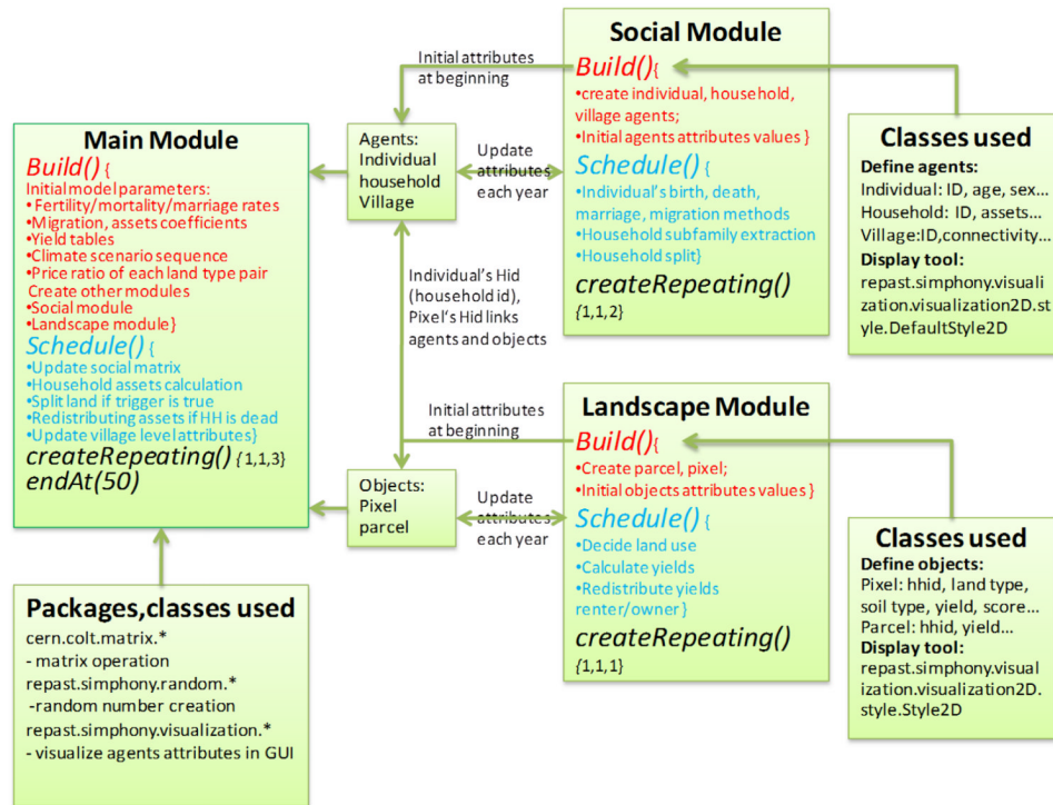
Figure 4. Primary program modules used in the Nang Rong ABM, with an emphasis on the Land Component portion of the model.
