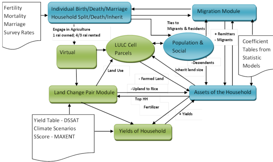
Figure 5. System operations of the Nang Rong ABM showing selected connectivity and process relationships of the Land Component portion of the model.
