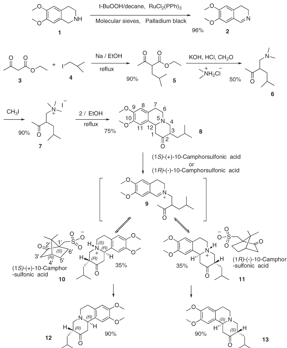
Scheme 1. Synthesis of TBZ Enantiomers
