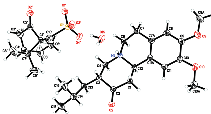
Figure 1. Structure and absolute configuration of (1S)-(+)-10-camphorsulfonate of (+)-TBZ ( 10 ) provided by X-ray crystallography: The absolute configuration was determined unambiguously from the anomalous data [Flack = -0.02(7) ]. The absolute configuration as reported by PLATON is C3 = R, N5 = S, C12 = R, C1' = S (from acid), and C4' = R (also from acid). For additional details, see the Supporting Information.
