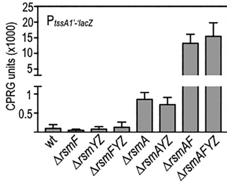
FIG 3 Control of tssA1' - lacZ translational reporter activity by the RsmAFYZ system. The indicated mutants carrying the tssA1' - lacZ translational reporter were cultured to mid-exponential phase and assayed for \beta -galactosidase activity by use of CPRG as a substrate.
