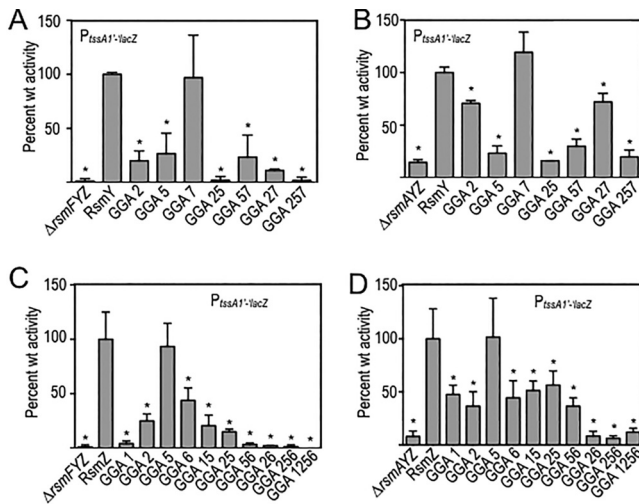
FIG 4 Regulation of RsmA and RsmF activities by mutant RsmY and RsmZ regulatory RNAs. The \Delta rsmFYZ (A and C) and \Delta rsmAYZ (B and D) mutants bearing the tssA1' - lacZ translational reporter were transformed with the indicated RsmY (A and B) or RsmZ (C and D) expression plasmids. Transformants were cultured to mid-exponential phase in the presence of 0.1% arabinose to induce expression of the respective RNAs and then assayed for \beta -galactosidase activity. Reported values represent the averages for at least three experiments, with standard errors indicated by error bars. The indicated statistically significant differences (*, P < 0.05 ) are relative to strains expressing either native RsmY (A and B) or RsmZ (C and D), normalized to 100% activity.
