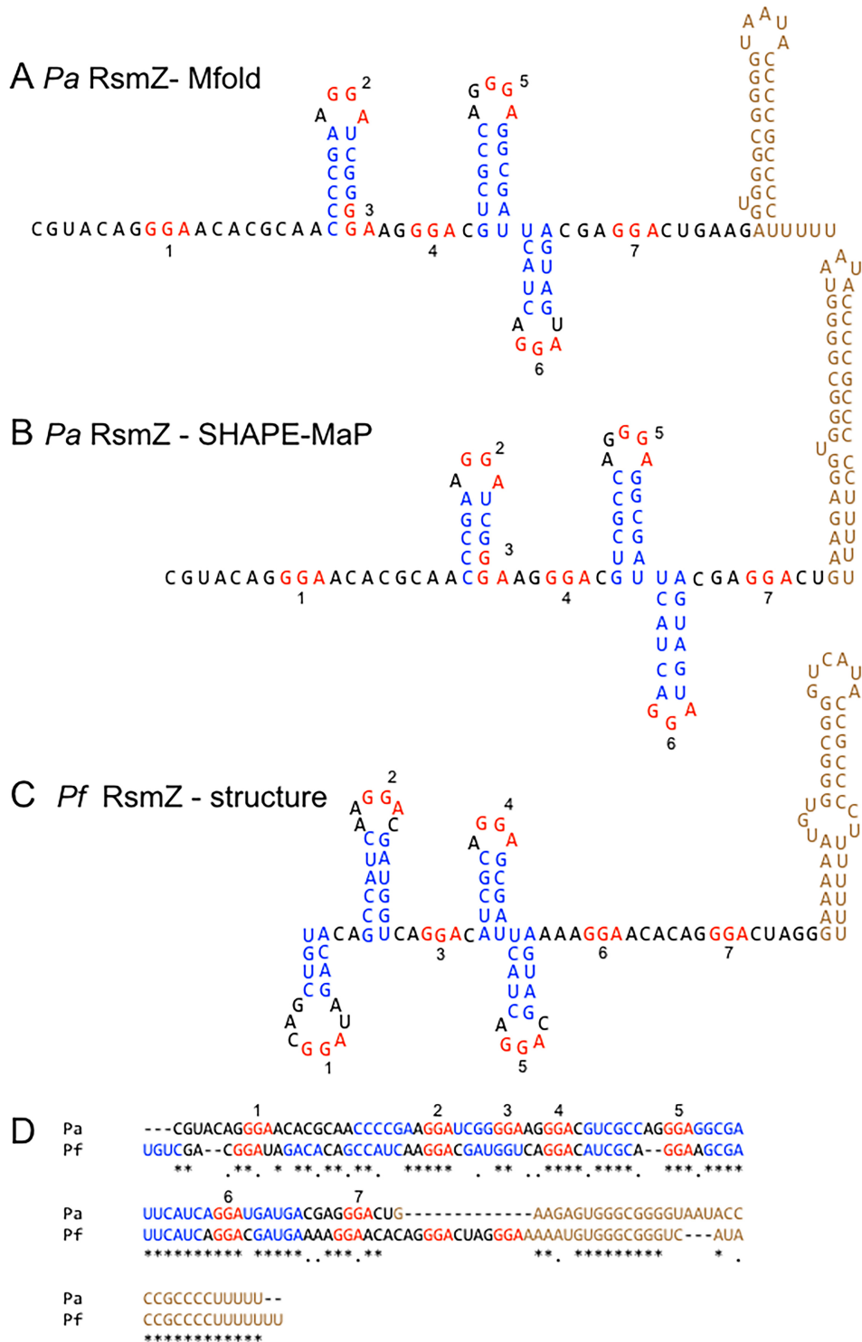
FIG 2 Predicted and determined structures of RsmZ. (A) Predicted Mfold structure for P. aeruginosa RsmZ. (B) SHAPE-MaP structure for P. aeruginosa RsmZ. (C) P. fluorescens RsmZ NMR structure. (D) Alignment of P. aeruginosa and P. fluorescens rsmZ sequences. GGA motifs are numbered 1 to 7 and highlighted in red. Stem structures are highlighted in blue, and terminator regions are shown in brown.
