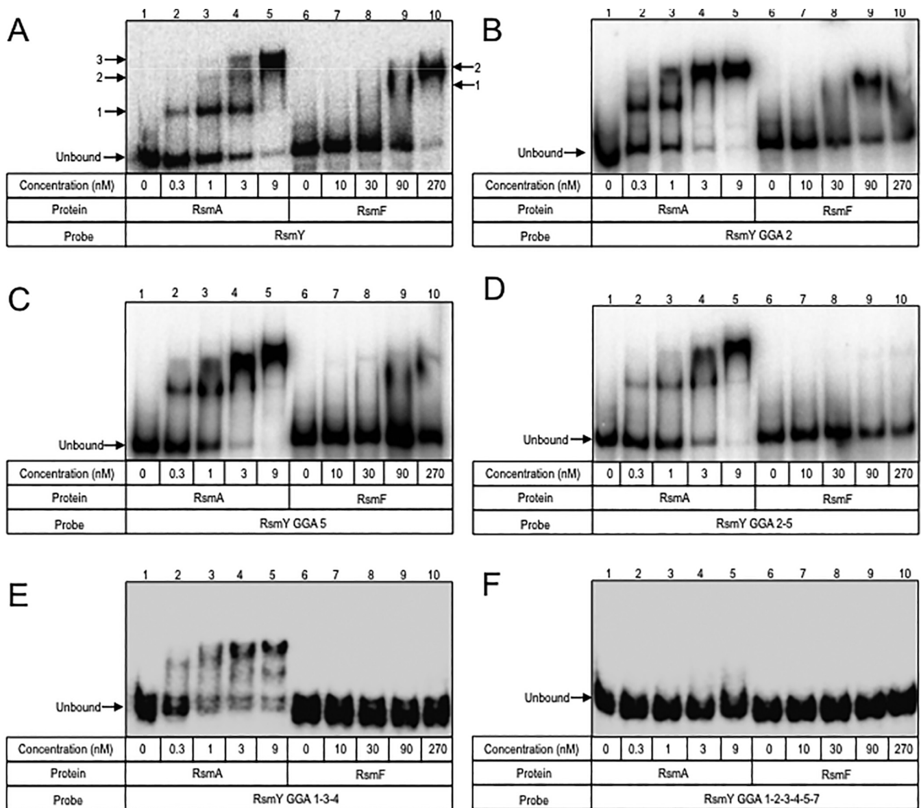
FIG 6 RsmA and RsmF binding to mutant RsmY RNAs. (A to F) The indicated RNAs were synthesized in vitro , radiolabeled, incubated with RsmA (lanes 1 to 5) or RsmF (lanes 6 to 10), and analyzed by nondenaturing polyacrylamide gel electrophoresis. Complexes formed upon RsmA or RsmF binding to native RsmY are indicated by arrows and numbered in panel A. Unbound RNA is indicated by an arrow in each panel.
