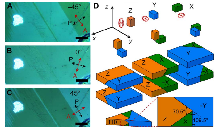
Fig. 1. Polarized light optical images and domain configurations in a \text{MAPbI}_3 single crystal (sample C). (A to C) Reflection-mode polarized optical micrographs (crossed Nicols) showing contrast reversal of domain groups as a function of sample rotation relative to the polarizer-analyzer (P-A) pair. At 0^\circ relative angle, the domain groups are indistinguishable, and, at 45^\circ and -45^\circ , the domain contrast is maximum; that is, \theta_e = 90^\circ . The red and black arrows indicate the analyzer orientation and polarizer orientation, respectively. The light intensity of a bright dust particle is insensitive to the sample rotation. Scale bars, 5 \mu\text{m} . (D) Permissible domains of the \text{MAPbI}_3 tetragonal phase. At the cubic-to-tetragonal transition, the tetragonal unit cell can form with the c axis aligned along any of the three axes ( x , y , and z ) of the parental cubic phase, leading to three possible configurations (X, Y, and Z). To preserve crystal integrity, the a axes of different domains must coincide (32), leading to six possible domain orientations that are characterized by domain walls intersecting at 0^\circ , 90^\circ , or 45^\circ in the principal planes of the parental phase and at \approx 70^\circ and \approx 110^\circ in the (110) plane.
