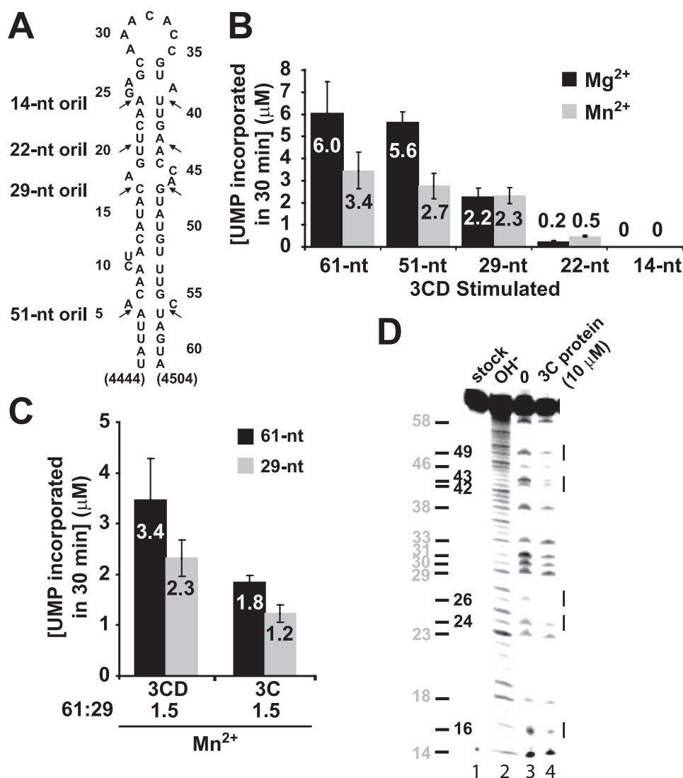
FIGURE 2. A 29-nt oril element and protein 3C are sufficient to direct specific and efficient VPg uridylylation in vitro . A , sites of oril truncation. PV orils containing stems of various lengths as indicated were produced by using in vitro transcription (61 and 51 nt) or chemical synthesis (29, 22, and 14 nt). B , a 29-nt oril is sufficient for VPg uridylylation in vitro . Shown is product formed in reactions containing oril templates of varying length (1 μM) in the presence of Mg 2+ (black bars) or Mn 2+ (gray bars) as the cofactor for PV 3Dpol. Reactions were stimulated using 3CD (1 μM) in the presence of 3D (1 μM) and the indicated RNAs (1 μM). The average of at least two independent experiments is reported along with the corresponding S.D. values. C , 3C is sufficient for VPg uridylylation in vitro . Shown is product formed in reactions containing the 61-nt (black bars) or 29-nt oril (gray bars) stimulated by using either 3CD or 3C. The average of at least two independent experiments is reported along with the corresponding S.D. values. D , footprint of 3C on oril. Shown is iodine cleavage of AMPαS-substituted 61-nt oril. Cleavage products were analyzed by denaturing PAGE. Shown is the phosphor image of the gel. Lane 1, untreated oril; lane 2, oril cleaved by alkaline hydrolysis; lane 3, iodine-treated oril in the absence of 3C; lane 4, iodine-treated RNA in the presence of 3C (10 μM). Sites of 3C binding are indicated by lines to the right of the gel. The position of the adenosine residues is indicated to the left of the gel.
