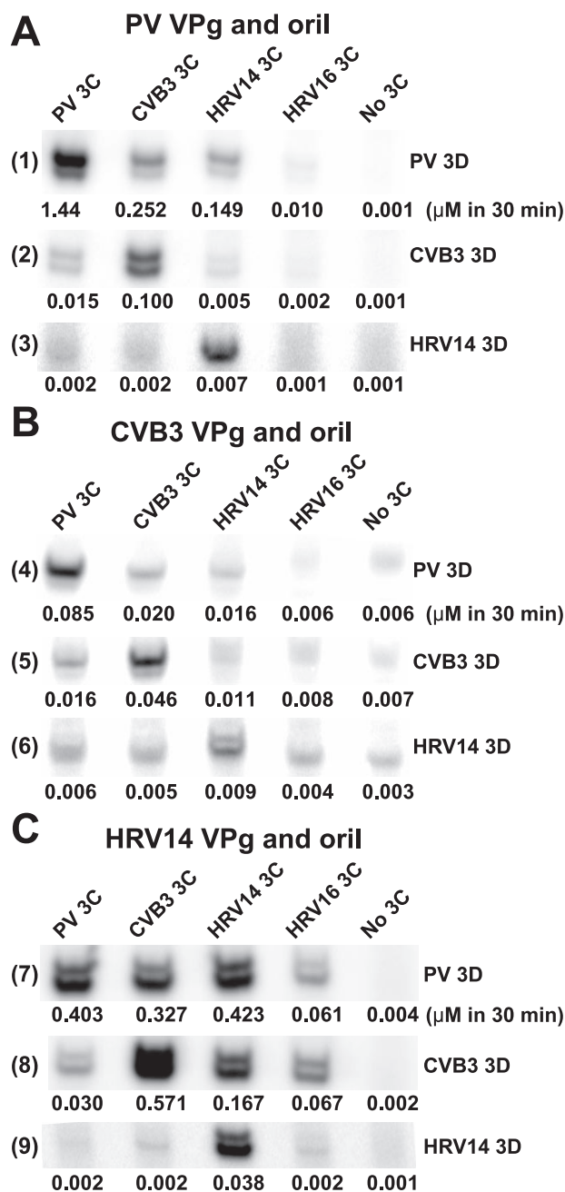
FIGURE 8. Evidence for a 3C-3Dpol interaction: Cognate 3C-3Dpol pairs are more efficient at VPg uridylylation independent of the origin of the VPg and oril. VPg uridylylation reactions contained cognate VPg-oril pairs from PV (A), CVB3 (B), or HRV14 (C). The source of 3C and 3Dpol is as indicated. Shown is a representative phosphor image of the VPg-pU(pU) products. Quantifications of UMP incorporation are indicated under each lane ( \mu\text{M} VPg-pU(pU) in 30 min). The S.E. value of the measurement did not exceed 20%. Reactions were performed in buffer (50 mM HEPES, pH 7.5, 5 mM magnesium acetate, 10 mM \beta -ME, 10% glycerol, 10 \mu\text{M} UTP, and 0.04 \mu\text{M} [ \alpha - ^{32}\text{P} ]UTP (6000 Ci/mmol)) at 30 ^{\circ}\text{C} for 30 min using 3D (1 \mu\text{M} for PV and CVB3, 10 \mu\text{M} for HRV14), 3C (1 \mu\text{M} ), VPg (10 \mu\text{M} ), and oril (1 \mu\text{M} ).
