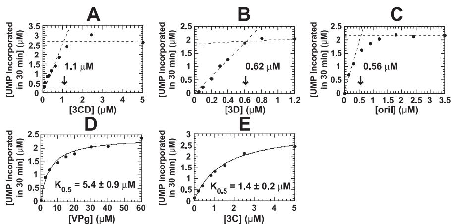
FIGURE 3. The active uridylylation complex contains one 3Dpol and two 3C(D) molecules per 29-nt RNA. Shown is product formed in reactions in which protein and nucleic acid components were titrated individually. Reactions were performed in buffer (50 mM HEPES, pH 7.5, 5 mM manganese acetate, 10 mM \beta -ME, 10% glycerol, 10 \mu M UTP, and 0.04 \mu M [ \alpha - ^{32} P]UTP (6000 Ci/mmol)) at 30 °C for 30 min using 3D, 3CD, and 29-nt oril at 1 \mu M and VPg at 50 \mu M unless they were being titrated. A , titration of 3CD. Lines defining the two phases of the curve were defined by linear regression, and the point of intersection was obtained algebraically. The intersection is 1.1 \mu M. B , titration of 3Dpol. The data were analyzed as described for 3CD titration. The intersection is 0.62 \mu M. C , titration of oril. The data were analyzed as described for 3CD titration. The intersection is 0.56 \mu M. D , titration of VPg. The data were fit to a hyperbola. The K_{0.5} value is 5.4 \pm 0.9 \mu M. E , titration of 3C. The data were fit to a hyperbola. The K_{0.5} value is 1.4 \pm 0.2 \mu M.
