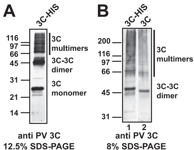
FIGURE 4. PV 3C can form dimers. A , cross-linking of His-tagged 3C. PV 3C containing a carboxyl-terminal His tag (1 \mu M) was incubated in reaction buffer at 30 °C for 15 min. Glutaraldehyde (1 mM) was added, and the reaction was incubated at 37 °C for 1 min, quenched with 2 \times SDS-PAGE dye, and analyzed by using 12.5% SDS-PAGE followed by Western blot analysis. B , cross-linking of “authentic” 3C. The experiment was performed as described above. An 8% gel was employed to resolve the multimers. Lane 1, 3C-His; lane 2, “authentic” 3C.
