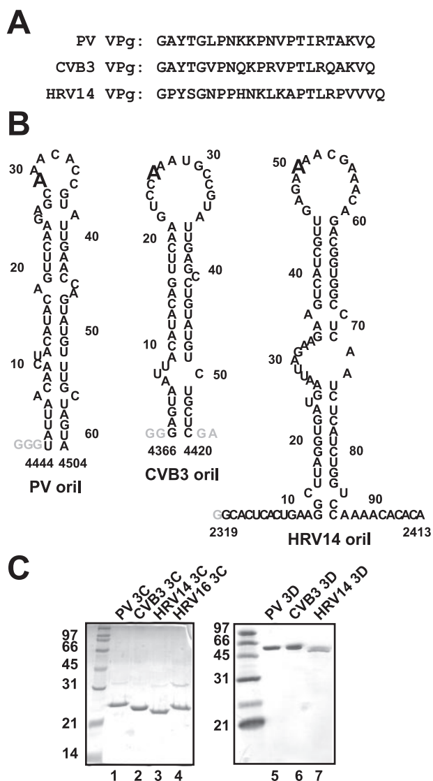
FIGURE 7. VPg uridylylation components employed in this study. A, VPg peptides. Only five of the 22–23 amino acids are strictly conserved. One of these is Tyr-3, the nucleophile employed for the first nucleotidyl transfer reaction. B, orils. Although structural differences are apparent among the three stem-loop RNAs, the orils of enteroviruses and rhinoviruses have been shown to be functionally exchangeable (3, 8, 10, 32), suggesting that structure is not the primary determinant for recognition by the initiation complex. The templating “A” located in the loop is in an enlarged font . C, purified 3C and 3Dpol proteins. SDS-PAGE analysis of 1.5 \mu\text{g} of each 3C and 1 \mu\text{g} of each 3D is shown (left and right polyacrylamide gels, respectively).
