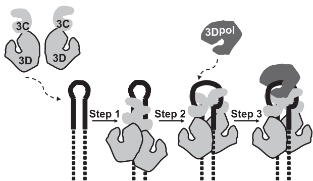
FIGURE 10. Assembly and organization of the VPg ribonucleoprotein complex. Step 1 , two 3CD molecules bind to oril with the 3C domains contacting the upper stem ( solid lines ) and the 3D domains contacting the lower stem ( dashed lines ). Step 2 , the 3C dimer opens the RNA stem by forming a more stable interaction with single strands forming the stem. Step 3 , 3Dpol is recruited to and retained in this complex by a physical interaction between the back of the thumb subdomain of 3Dpol and a surface of one or both 3C subdomains of 3CD.
