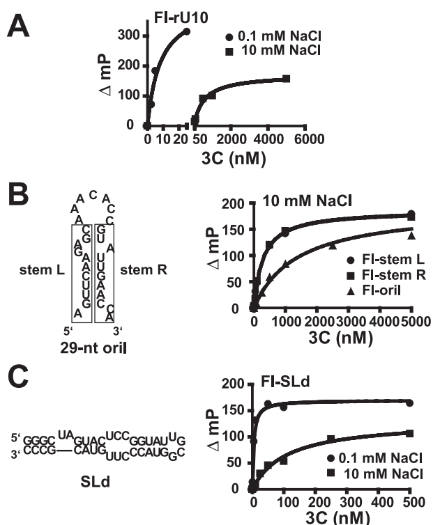
FIGURE 5. RNA binding by PV 3C measured by using fluorescence polarization. A , 3C binds single-stranded RNA and is sensitive to salt concentration. 3'-Fluorescein-labeled rU10 (FL-rU10) RNA was titrated with 3C in the presence of 0.1 and 10 mM NaCl. Binding was detected as a change in fluorescence polarization ( mP ) in a Beacon instrument. The data were fit to a hyperbola. B , 3C binds to single-stranded oril RNA fragments better than to intact oril. The intact oril employed is shown. The rectangles on the left and right define the RNA sequences of "stemL" and "stemR" single-stranded RNAs, respectively. All RNAs were labeled at the 3'-end with fluorescein. Experiments were performed as described above in the presence of 10 mM NaCl. C , 3C binding to Sld is tight. The 5'-end of PV RNA contains a cis-acting element (oril) that contains a high affinity binding site for 3CD termed Sld. The sequence and secondary structure are shown on the left . Sld RNA was labeled at the 3'-end with fluorescein. Experiments were performed as described above in the presence of 0.1 and 10 mM NaCl.
