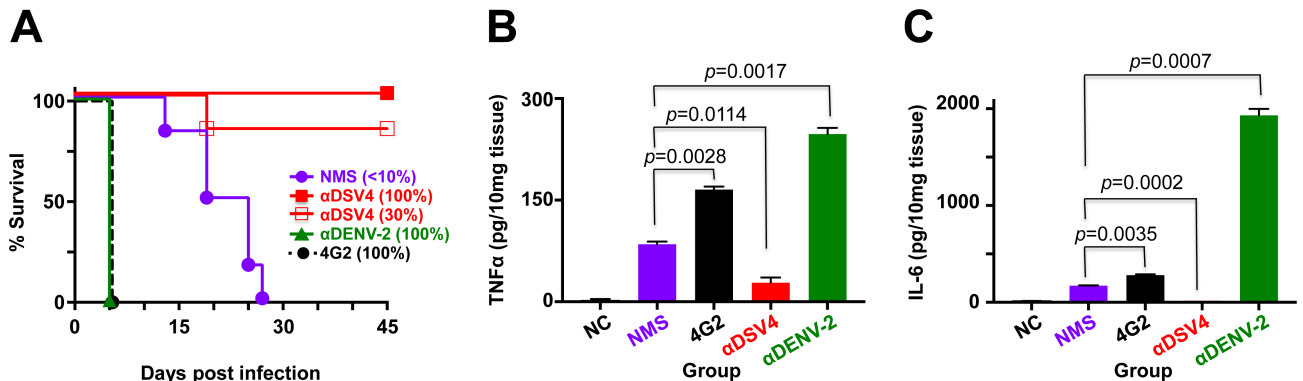
Fig 4. Lack of ADE by anti-DSV4 antibodies correlates with protective efficacy in AG129 mice. (A) Groups ( n = 6 ) of AG129 mice were challenged with sub-lethal dose of DENV-2 S221 pre-incubated with normal mouse serum (NMS) or in vitro -generated ICs of the same sub-lethal dose of DENV-2 using either sub-neutralizing amounts of anti-DSV4 antiserum [ \alpha DSV4 (30%)], or fully neutralizing amounts of anti-DSV4 antiserum [ \alpha DSV4 (100%)], anti-DENV-2 antiserum [ \alpha DENV-2 (100%)] or mAb 4G2 [4G2 (100%)], and monitored for survival. Survival curves for different groups at the 100% mark have been slightly displaced to make them visible. Survival rates of \alpha DSV4 (30%) IC group ( p = 0.0009 ) and \alpha DSV4 (100%) IC group ( p = 0.0009 ), compared to that of the 4G2 (100%) group was significant, based on the Log-Rank (Mantel-Cox) test; with respect to the NMS group (challenged with free DENV-2 S221) also, survival was significantly higher for \alpha DSV4 (30%) group ( p = 0.006 ) and the \alpha DSV4 (100%) group ( p = 0.0006 ). (B) Groups of AG129 mice ( n = 3 ) were challenged as described in panel A with the exception that the \alpha DSV4 (30%) IC group was replaced with an untreated group to serve as the negative control (NC). Three days post-inoculation mice were euthanized, small intestines dissected out after perfusion and homogenized. Clarified homogenates were used for the determination of TNF- \alpha using a commercial ELISA kit with purified recombinant murine TNF- \alpha as the reference. (C) The same experiment as in panel B, except that the clarified homogenates were used for IL-6 determination using a commercial ELISA kit with purified recombinant murine IL-6 as the reference. Data shown in panels 'B' and 'C' are mean values ( n = 3 ) with the bars denoting standard deviation. Unpaired t test was used to derive the p values shown in panels B and C.
