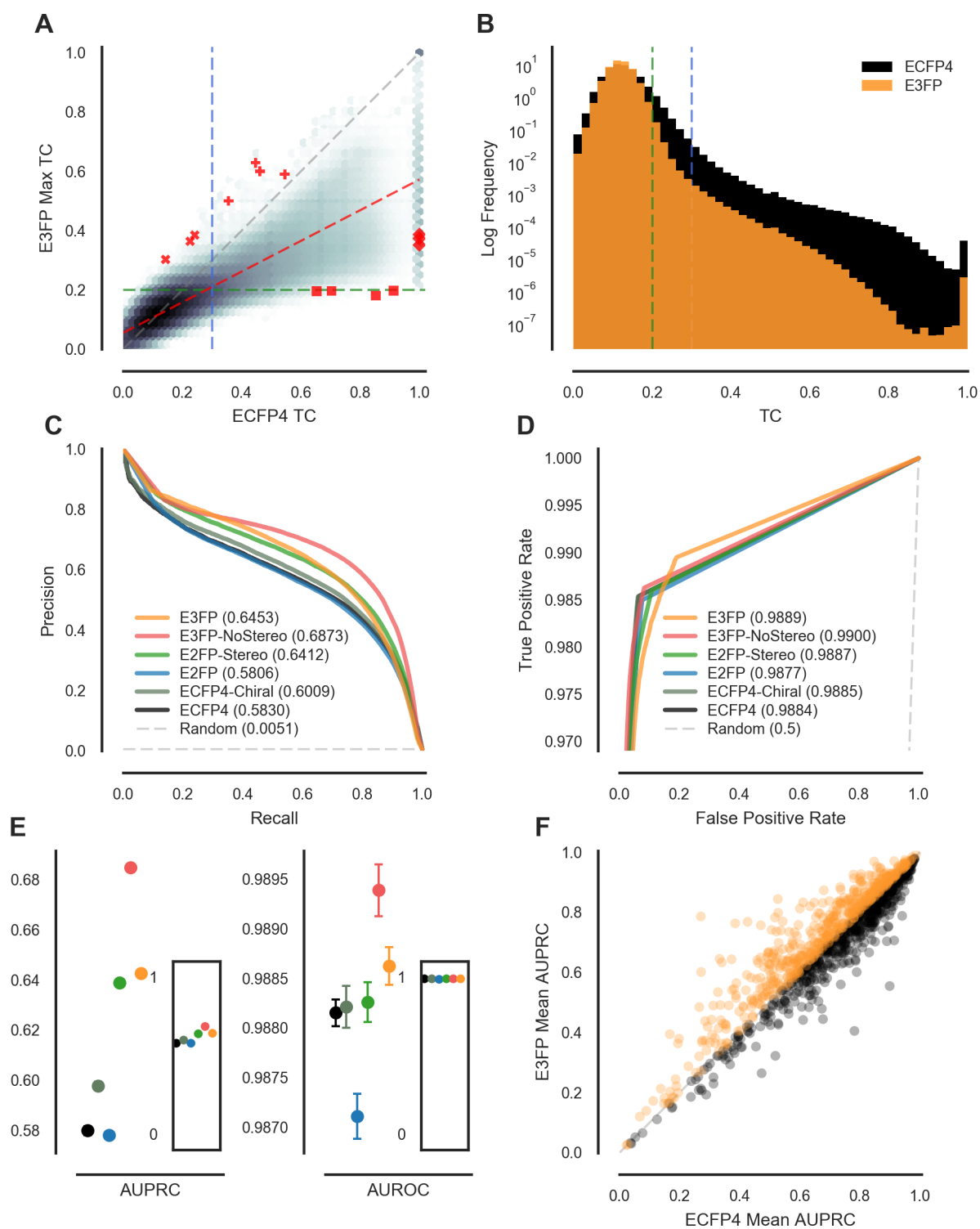
Figure 2. Comparative performance of E3FP and ECFP4. For all pairs of 308315 molecules from ChEMBL20, (A) log density plot summarizing 48 billion maximum Tanimoto coefficients (TC) calculated between E3FP conformer fingerprint sets versus corresponding TC by ECFP4 fingerprints. The dotted red line is a linear least-squares fit. Optimal SEA TC cutoffs for E3FP (green) and ECFP4 (blue) are dotted lines. Red markers indicate examples in Figure 3. (B) Histograms of TCs from (A). (C) Combined precision-recall (PRC) curves from five independent 5-fold cross-validation runs using 1024-bit E3FP, E3FP without stereochemical identifiers (E3FP-NoStereo), E3FP without stereochemical identifiers or nearby unbound atoms (E2FP), E3FP without nearby unbound atoms (E2FP-Stereo), ECFP4, and ECFP4 with distinct bond types encoding chirality (ECFP4-Chiral). Only the PRC of the highest AUC fold is shown. (D) Combined highest-AUC ROC curves for the same sets as in (C). (E) Results of bootstrapping AUCs as in Table 1. Dots indicate mean AUC, and whiskers standard deviations. Insets show absolute scale. (F) Target-wise comparison of mean AUPRCs using E3FP versus ECFP4.
