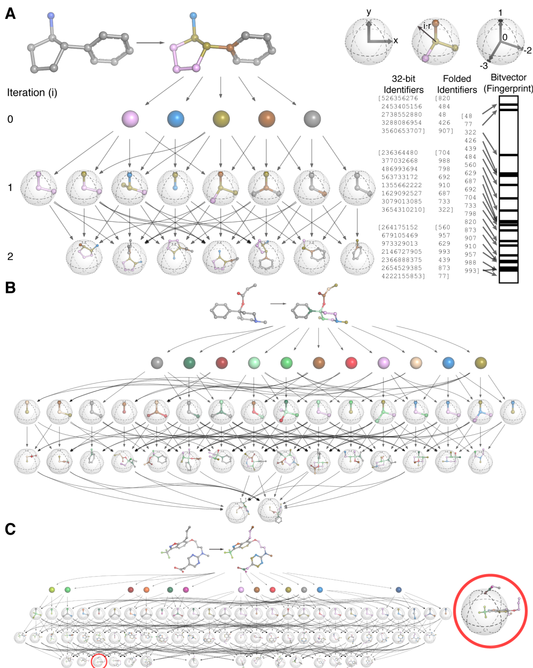
Figure 1. Diagram of information flow in the E3FP algorithm. (A) Overview of fingerprinting process for cypenamamine. At iteration 0, we assign atom identifiers using a list of atomic invariants and hash these into integers (shown here also as unique atom colors). At iteration i , shells of radius i \cdot r center on each atom (top right). The shell contains bound and unbound neighbor atoms. Where possible, we uniquely align neighbor atoms to the xy -plane (top right) and assign stereochemical identifiers. Convergence occurs when a shell's substructure contains the entire molecule (third from the right) or at the maximum iteration count. Finally we “fold” each iteration’s substructure identifiers to 1024-bit space. (B) Overview of fingerprinting for alphaprodine. (C) Overview of fingerprinting for a large, flexible molecule (CHEMBL210990; expanded in Supporting Information, Figure S1). A three-dimensional substructure can consist of two disconnected substructures and their relative orientations (right).
