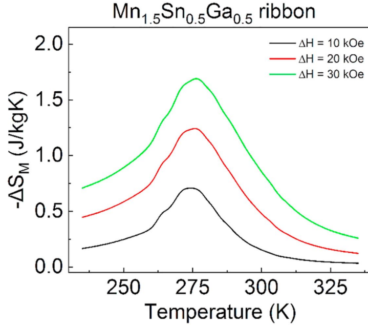
Fig. 7. Magnetic entropy change ( -\Delta S_M ) as a function of temperature for \text{Mn}_{1.5}\text{Sn}_{0.5}\text{Ga}_{0.5} as-quenched ribbons.
