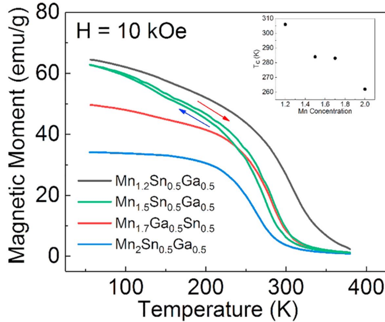
Fig. 2. Thermomagnetic curves of as-quenched \text{Mn}_{2-x}\text{Sn}_{0.5}\text{Ga}_{0.5} ( x=0, 0.3, 0.5, 0.8 ) ribbons, the inset shows the T_c as a function of Mn concentration.
