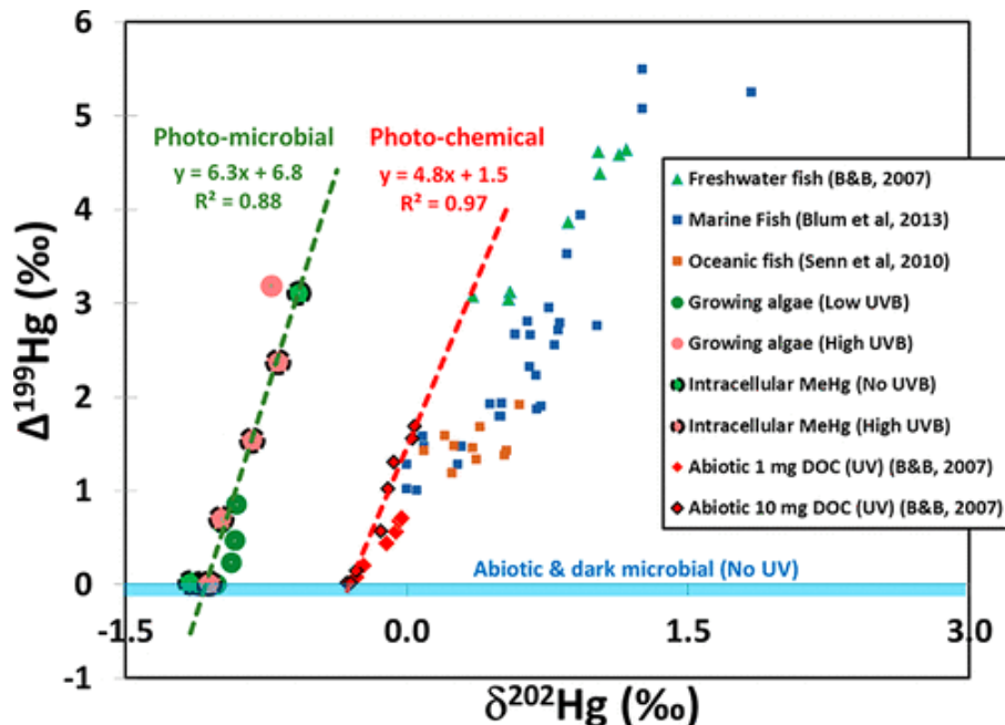
Figure 4. Mass independent ( \Delta^{199}\text{Hg} ) and mass dependent ( \delta^{202}\text{Hg} ) signatures in fish versus fractionation during photochemical and photomicrobial processes. A comparison of marine(26,27) and freshwater fish(29) isotopic data with stable isotopic fractionation during degradation of MeHg by photomicrobial (algal) and UV-mediated photochemical processes(29) shows that photomicrobial processes could contribute toward the accumulation of odd isotope-enriched MeHg in marine consumers. The photomicrobial and photochemical regression lines are based on all four photomicrobial demethylation experiments reported in this figure and abiotic photochemical reduction with 10 mg C/L,(29) respectively. The starting isotopic composition of MeHg stock used in our study is lighter than the standard used for isotopic analysis.
