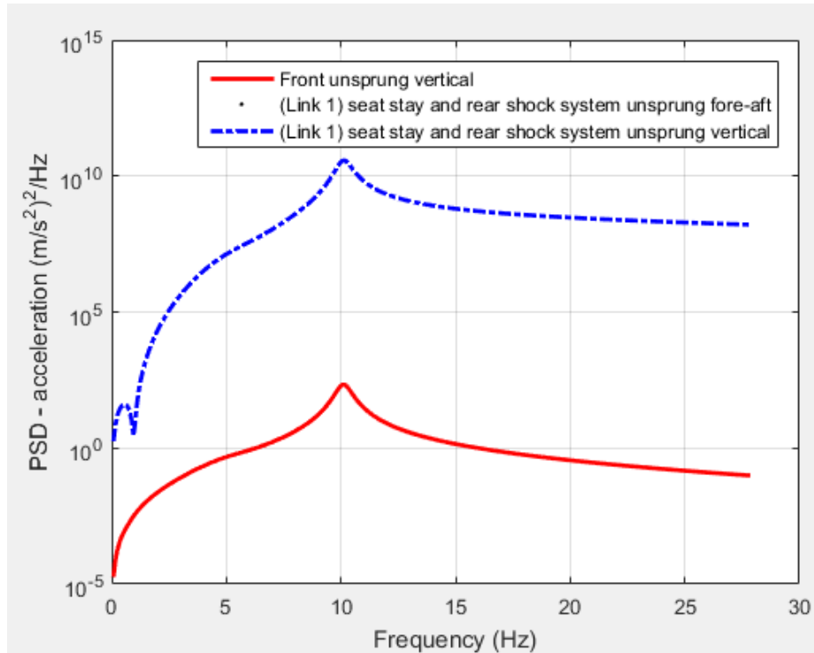
Figure 4.11 - PSD Plot (Front Unsprung Mass, Rear Shock and Seat Stay System Fore-aft, and Rear Shock and Seat Stay System Vertical)
