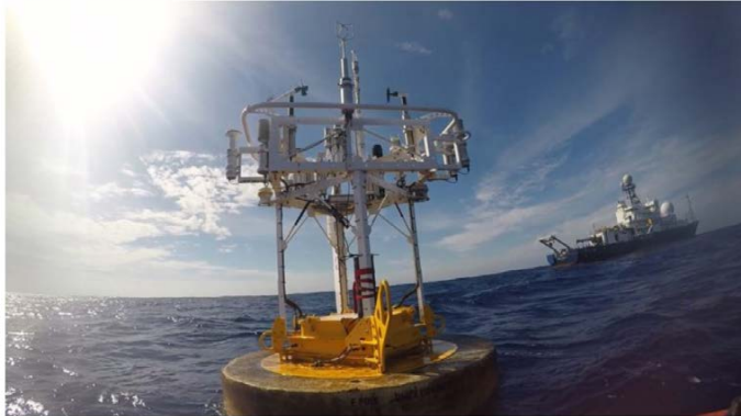
WHOI Mooring Buoy (credit Ray Graham).
