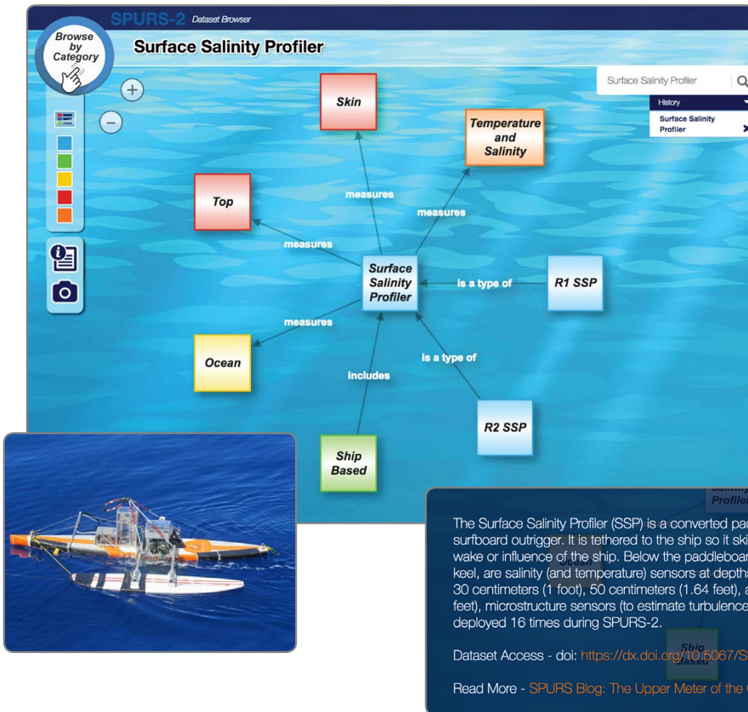
FIGURE 3. An expanded view of the visualized ontology based on a user click of the term “Surface Salinity Profiler.” Properties measured by the central term (e.g., “Top,” “Skin,” “Ocean,”) are placed at the ends of arrows. Conversely, arrows associated with broader categories (“Ship-Based”) lead to the central term. An image (lower left), a description of a data set, and a blog post link (lower right) provide context to enhance the user’s understanding.
