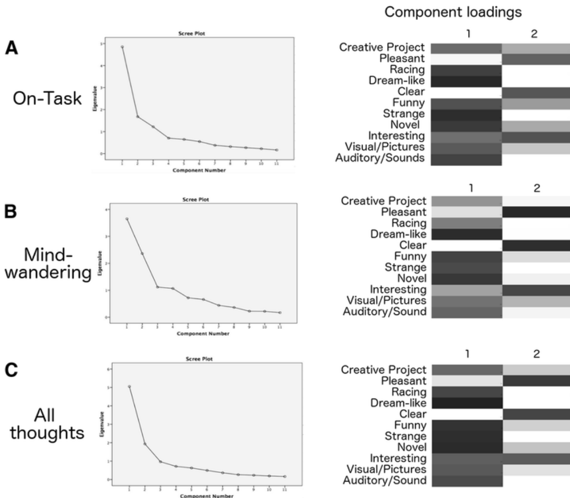
Figure 2. Scree plots and component loadings for the principal components analysis on the content variables. Results are shown when the analysis was performed on (A) on-task responses only, (B) mind wandering only, and (C) all thoughts.
