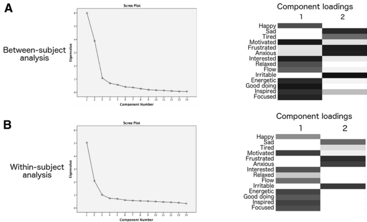
Figure 1. Scree plots and component loadings for the principal components analysis on the affect variables. Results are presented both when the analysis was performed at (A) a between-subjects level, and (B) a within-subject level.
