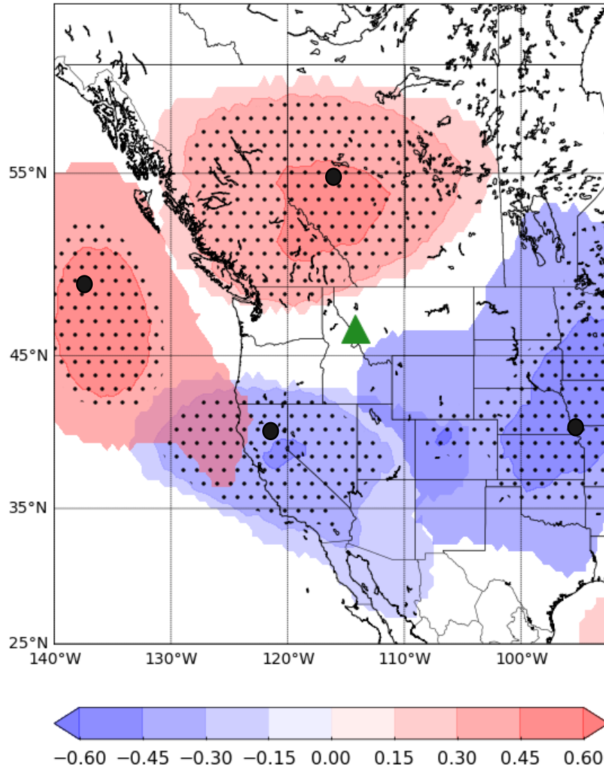
Figure 3 Spatial relationship (Pearson) between the BEST tree-ring chronology and upper-level (500 hPa) zonal and meridional flow from the North American Regional Reanalysis dataset (1979-2015). Colors indicate r values and black gridpoints indicate significance ( p= 0.01 ). Large black dots indicate the four locations of our climate reconstruction.
