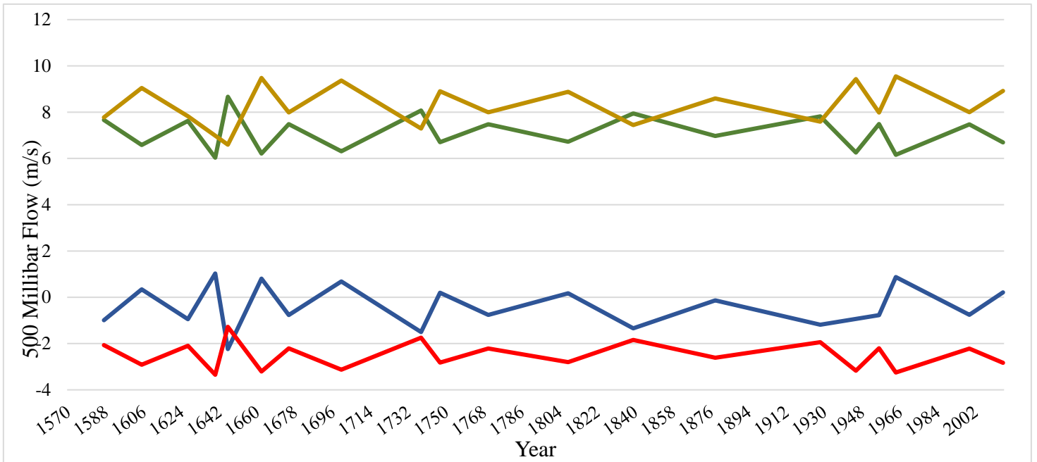
Figure 5 North (gold), south (green), east (red), and west (blue) Rodionov regime shifts from the upper-level (500 hPa) climate reconstructions. The slope of the lines was generated by connecting the mean values of the identified regimes.
