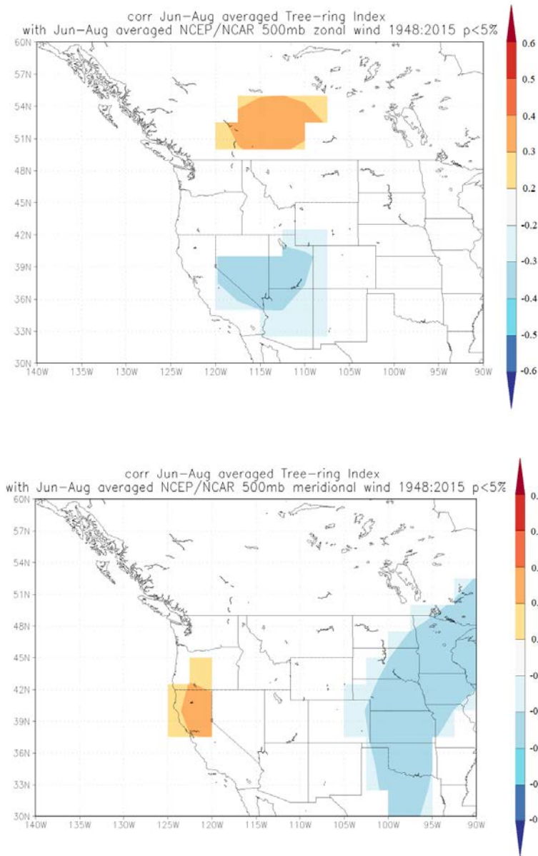
Figure 2 Significant ( p < 0.05 ) spatial pattern correlations between the COMBO tree-ring chronology and a. zonal wind (500 hPa) and b. meridional wind (500 hPa) from the NCEP/NCAR Reanalysis 1 dataset (1948-2015).
