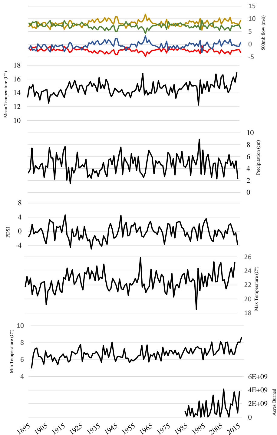
Figure 7 Temporal pattern (1895-2015) of a. north (gold), south (green), east (red), and west (blue) climate reconstruction, b. Montana Climate Division 1 mean temperature (JJA), c. Montana Climate Division 1 precipitation (JJA), d. Montana Climate Division 1 Palmer Drought Severity Index (August), e. Montana Climate Division 1 maximum temperature (JJA), f. Montana Climate Division 1 minimum temperature (June), and g. Montana and Idaho hectares burned (August).
