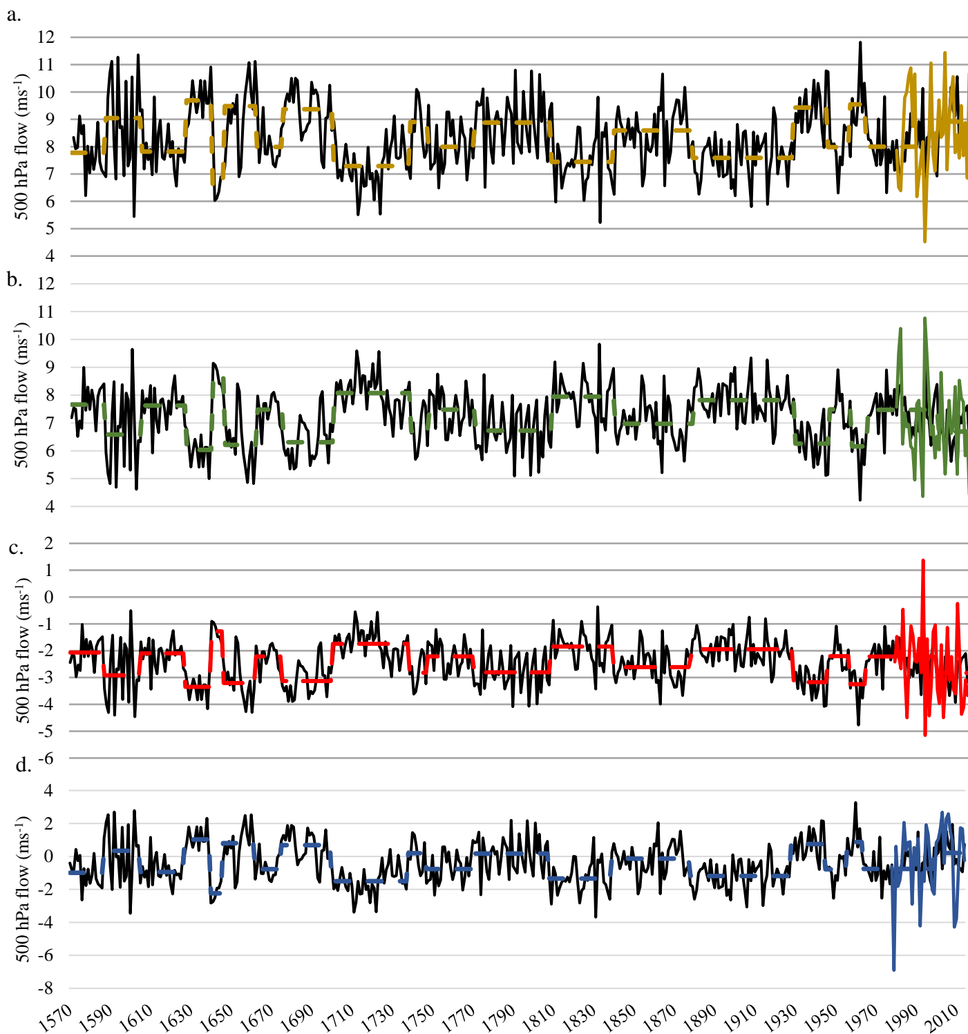
Figure 4 Climate reconstructions (solid black lines) of upper-level (500 hPa) atmospheric flow from 1571 to 2015 using the BEST tree-ring chronology for the four cardinal (a. north, b. south, c. east, and d. west) gridpoints having the strongest relationship between standardized radial tree growth and 500 hPa flow in the instrumental record (1979-2015). Solid color lines depict the actual 500 hPa flow and the dashed lines identify significant ( p < 0.05 ) regime shifts in the 500 hPa flow using the Rodionov regime shift test.
