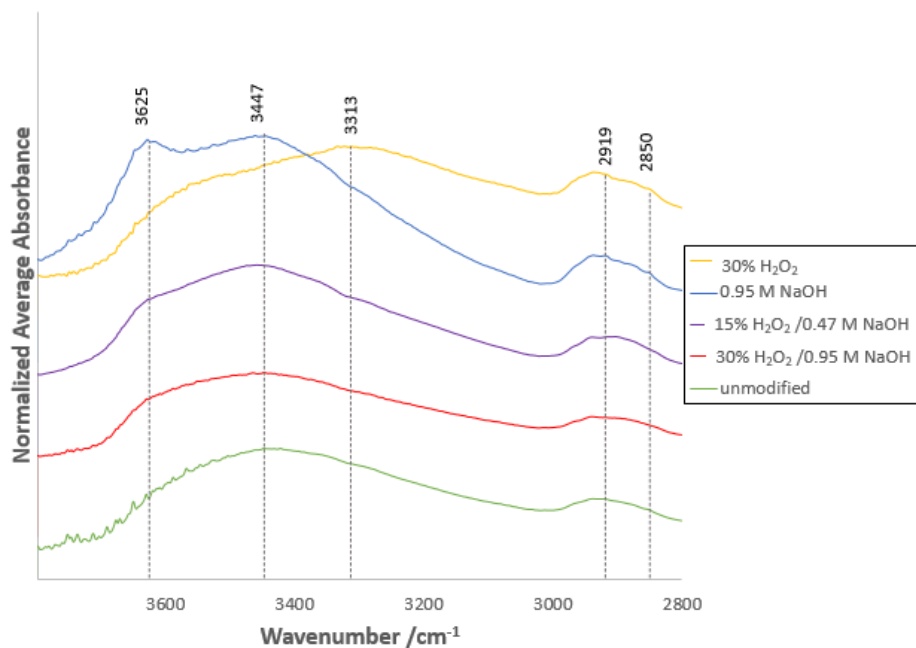
Figure 9. FT-IR spectra of unmodified and modified HD hulls from 3800-2800 \text{cm}^{-1} .
