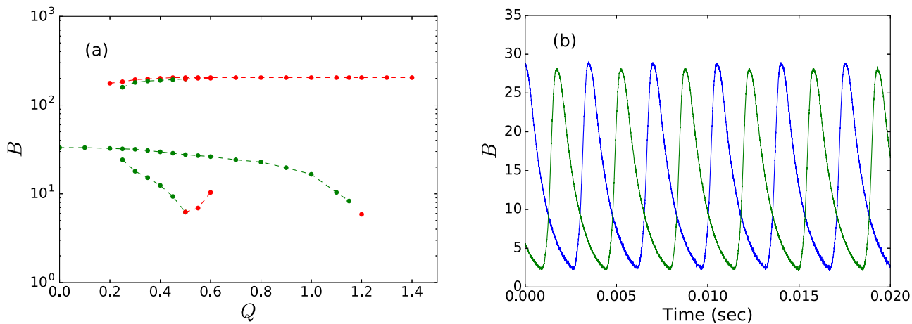
FIG. 4. Circuit measurements for two QS-coupled repressilators ( n = 2.8, \alpha = 204, \kappa = 17.8 ). (a) Q continuation showing stable steady-states (red) and stable limit cycles (green). (b) Time series showing APLC for Q = 0.4 . B values were calculated from measured voltages. Note that the APLC is continuously stable from Q = 0 to 1.15.
