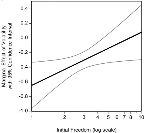
Figure 2: Marginal Effect of Volatility, Conditional on Initial Freedom (Table 2, Column 2)
