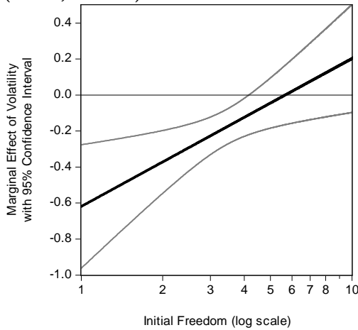
Figure 3: Marginal Effect of Volatility, Conditional on Initial Freedom (Table 2, Column 4)
