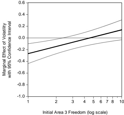
Figure 6: Marginal Effect of Volatility, Conditional on Initial Area 3 Freedom (Table 3, Column 3)
