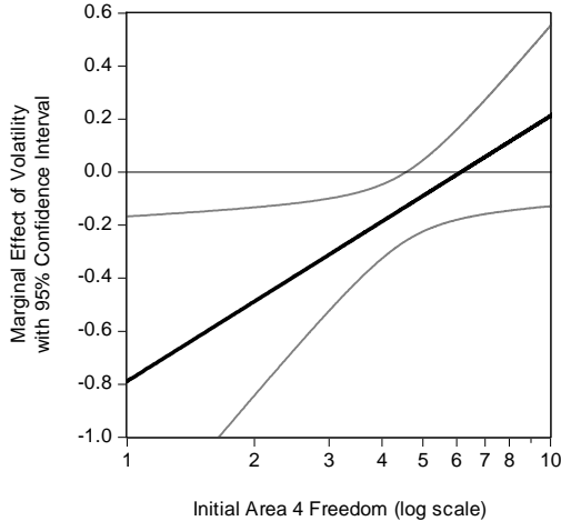
Figure 7: Marginal Effect of Volatility, Conditional on Initial Area 4 Freedom (Table 3, Column 4)
