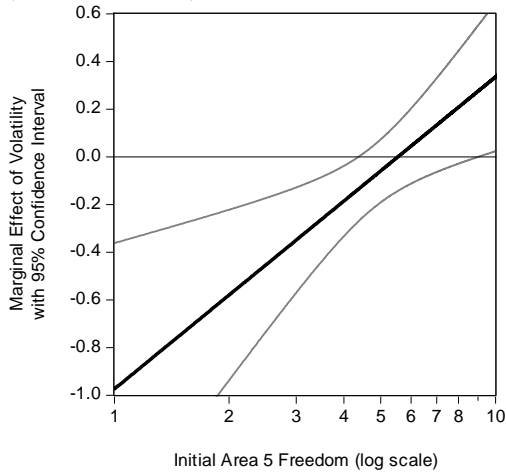
Figure 8: Marginal Effect of Volatility, Conditional on Initial Area 5 Freedom
