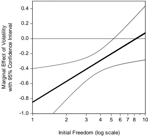
Figure 1: Marginal Effect of Volatility, Conditional on Initial Freedom (Table 2, Column 1)
