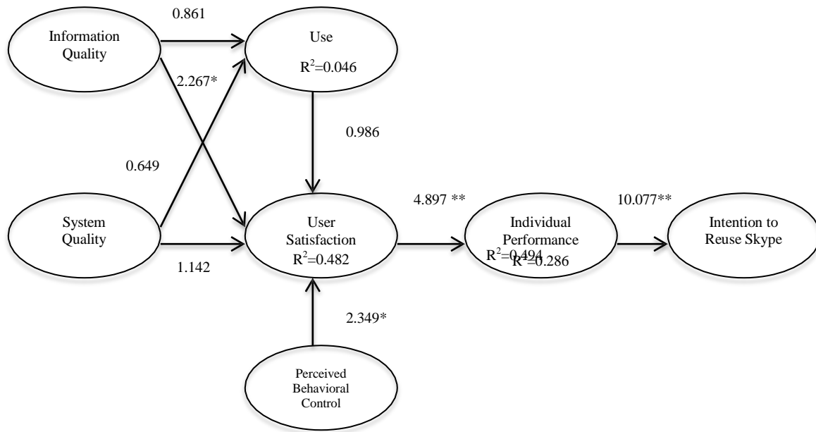
Figure 3. Path Analysis Results
