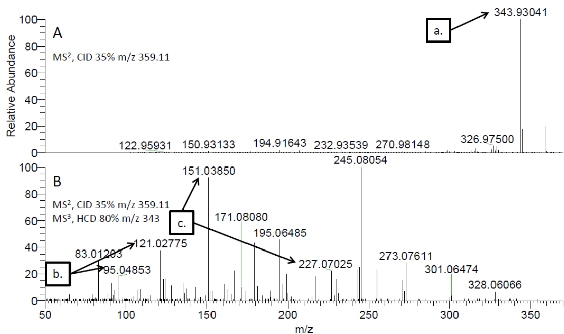
Figure 4.2. Sample MS 2 Data (4.2A) and MS 3 Data (4.2B) Derived from the Precursor Ion m/z 359.11.
