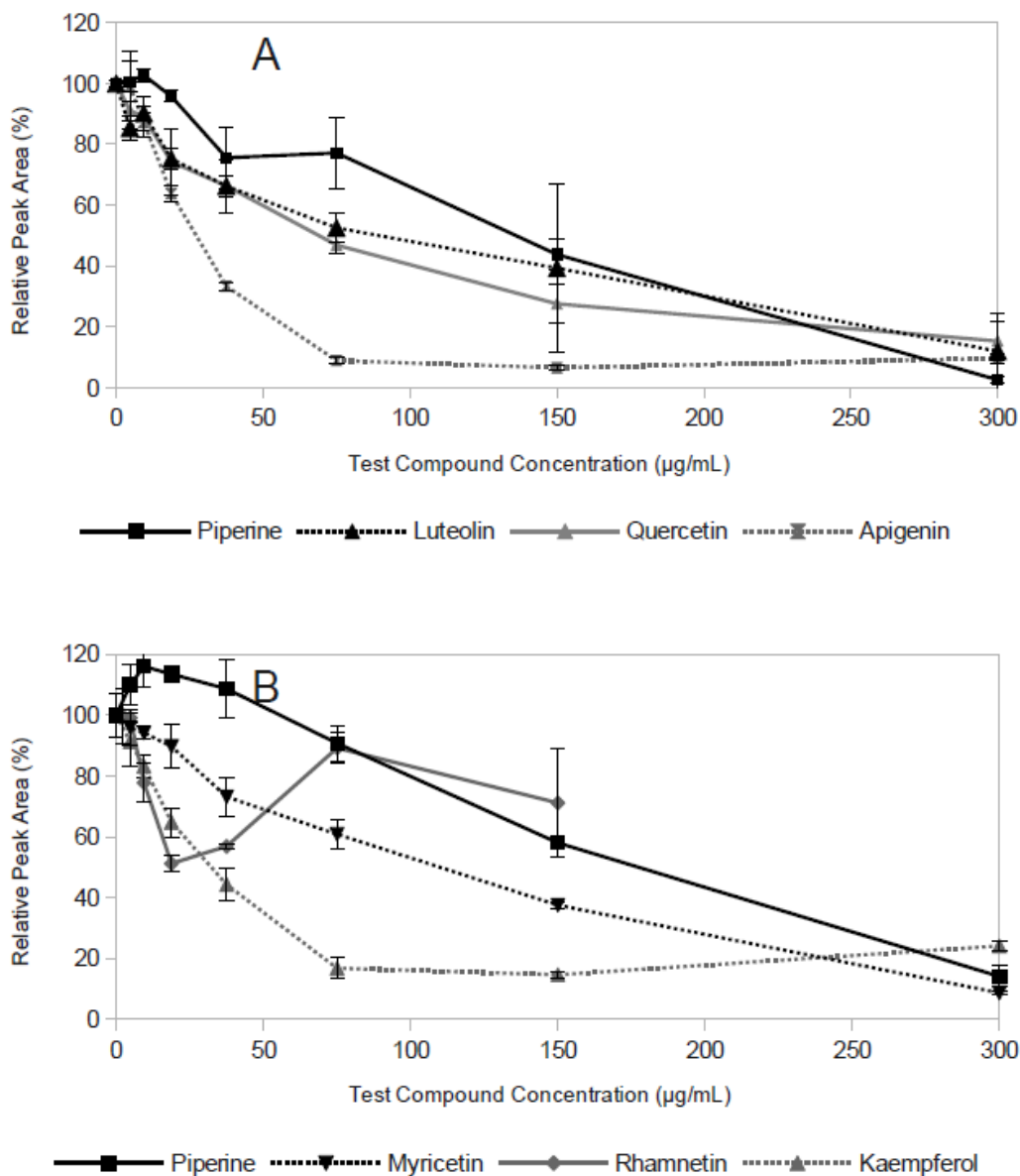
Figure 2.4. Efflux Pump Inhibitory Activity of 6 Flavonoids (Luteolin, Quercetin, Apigenin, Myricetin, Rhamnetin and Kaempferol) Compared to that of Piperine, as Indicated by LC-MS Measurement of Residual Ethidium Bromide in Spent Broth After a 30 Min Incubation.
