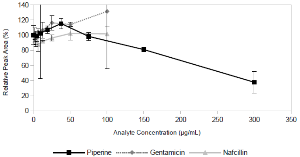
Figure 2.7. Efflux Pump Inhibitory Data Generated Via the Mass Spectrometry-Based Assay Performed on the Known Antibiotic Compounds Gentamicin and Nafcillin.
