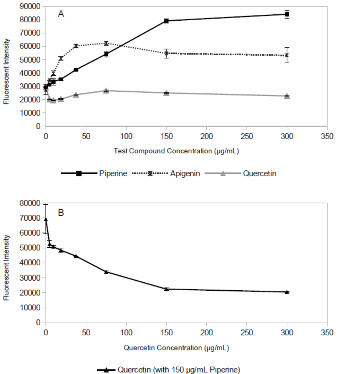
Figure 2.2. Change in Fluorescence Due to Ethidium Accumulation by S. aureus in the Presence of Putative Inhibitors. (A) Dose-response curves for the flavonoids apigenin and quercetin. (B) Fluorescence observed for 150 µg/mL piperine in the presence of increasing concentrations of quercetin. Decrease in fluorescence with increasing quercetin concentration in (B) can be attributed to fluorescence quenching by the flavonoid. Data points represent the mean of triplicate measurements (biological replicates), vertical bars represent standard deviation.
