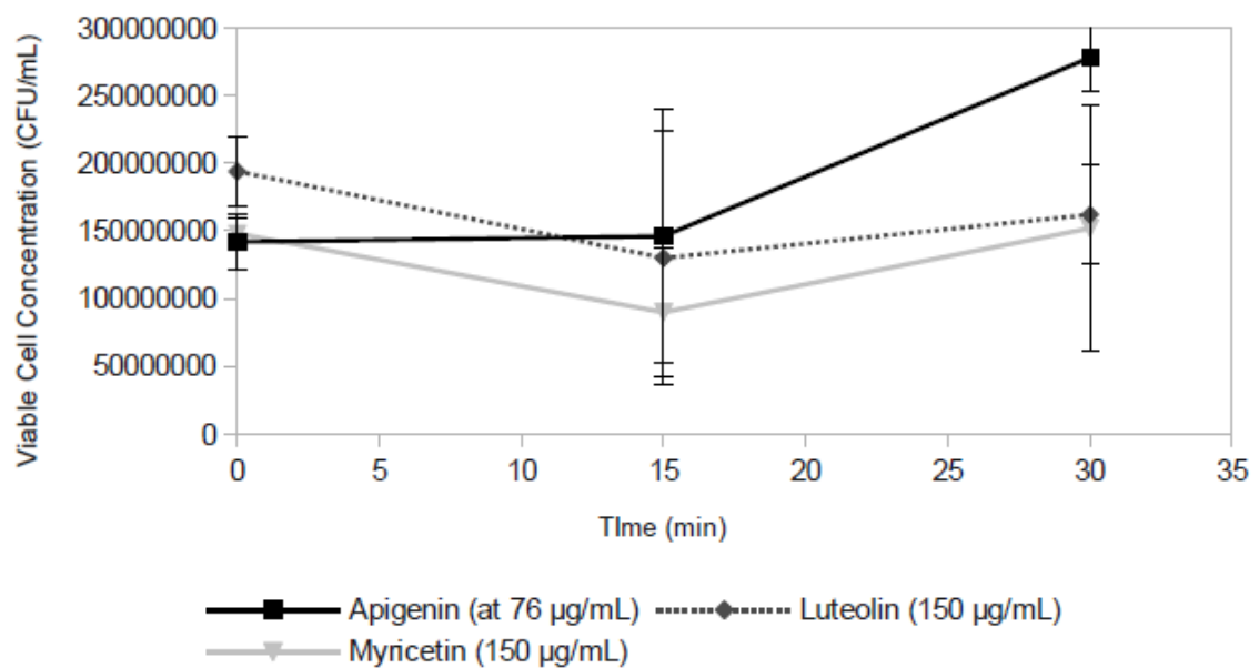
Figure 2.6. Time Series Data Evaluating the Viability of Staphylococcus aureus Cultures Exposed to Experimental Conditions.
