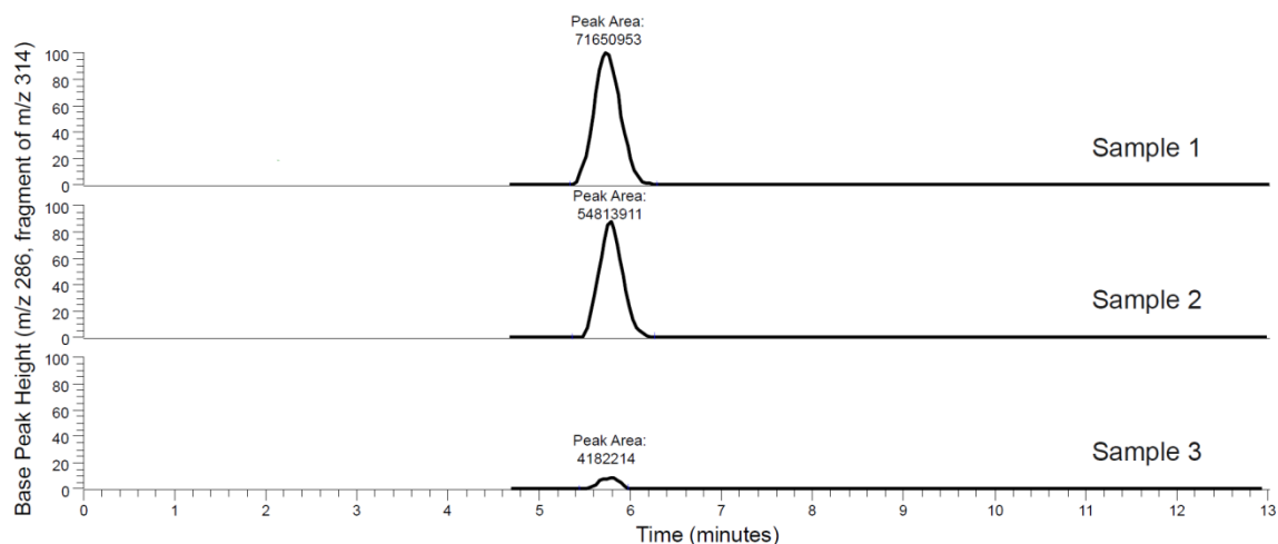
Figure 2.3. Representative Selected Chromatograms of Filtered, Spent Broth Showing a Peak for the Ethidium Ion (MS-MS Transition of m/z 314 to 286). Sample 1 is the negative control ( S. aureus cultured for 30 min in Mueller Hinton broth with 1.25 \mu\text{g}/\text{mL} ethidium bromide and 10% DMSO). Samples 2 and 3 were cultured under the same conditions as sample 1 with the addition of 75 \mu\text{g}/\text{mL} and 300 \mu\text{g}/\text{mL} piperine, respectively. All three peaks are normalized to a signal intensity of 3.45 \times 10^6 . As piperine is added, efflux pumps are blocked, trapping the ethidium inside the cells and decreasing the quantity of ethidium (as indicated by the area of the ethidium peak) in the spent broth.
