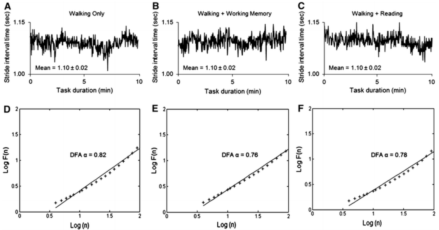
Fig. 1 Stride interval time series for one participant in each of the three conditions ( a , b , c ) and the corresponding DFA plots for each time series ( d , e , f )
