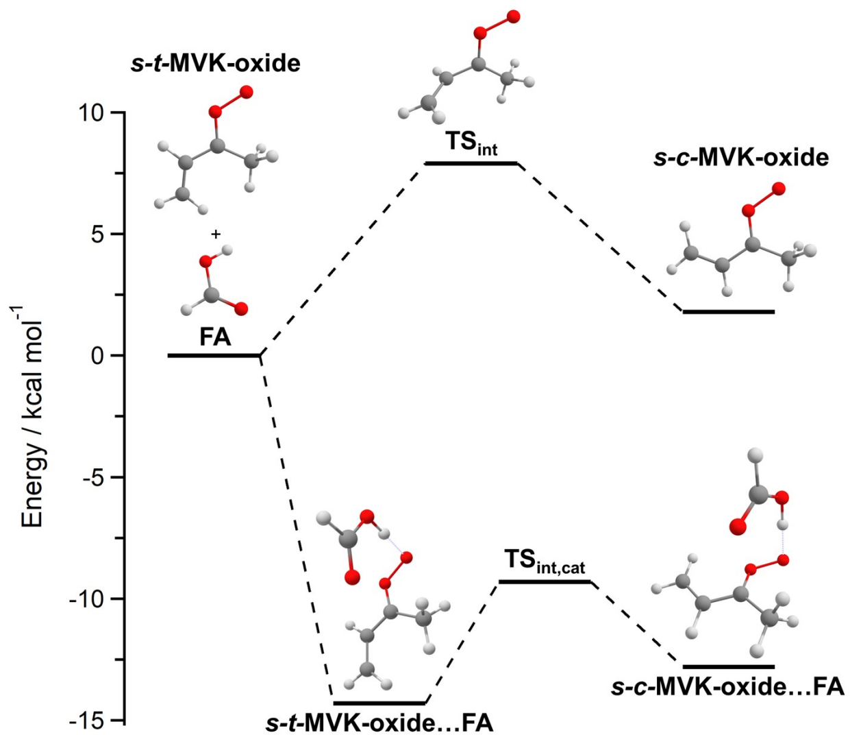
Figure S2. Reaction coordinate showing the barrier (TS int ) for interconversion between syn-trans and syn-cis configurations of MVK-oxide. A pre-reactive complex (PRC) formed between MVK-oxide and formic acid substantially lowers the barrier (TS int,cat ) and provides a route for rapid interconversion between trans ( s-t ) and cis ( s-c ) forms.
